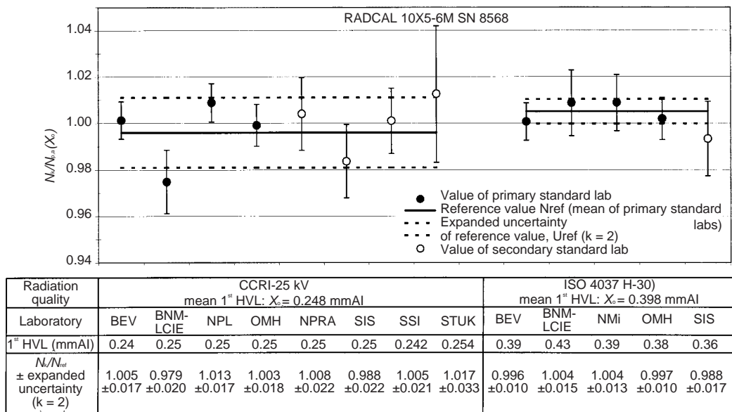
Figure 15. Ratio of air kerma calibration coefficients N_k and the value of the polynomial regression N_{p,a}(x_0) of all air kerma calibration coefficients at the mean 1st HVL x_0 of radiation qualities defined by the CCRI and the international standard ISO 4037-1:1996 (high air kerma rate series) at a constant tube voltage for Radcal chamber. Note: The mean 1st HVL was calculated from the 1st HVL of radiation qualities from primary standard laboratories.
