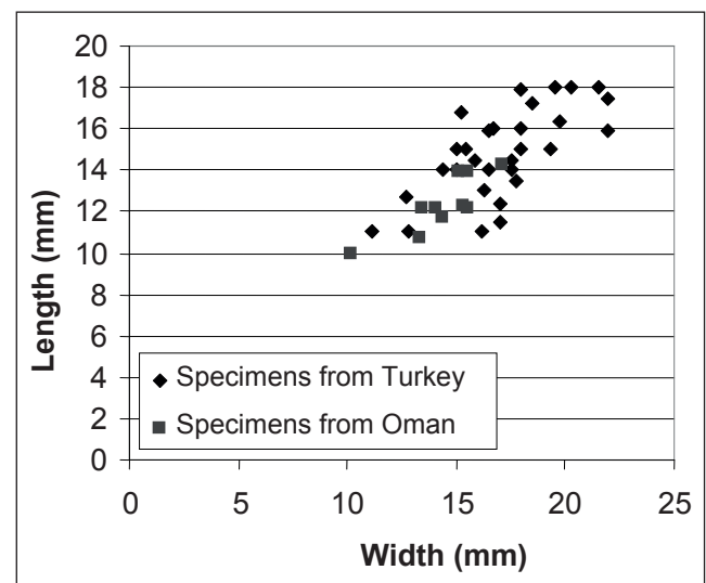
Fig. 8 - Width vs. length diagram of the specimens of Bilotina yanagidai from Oman (Angiolini in Angiolini & Bucher 1999), and those from Turkey; the latter seem to reach a larger size than those from Oman.
