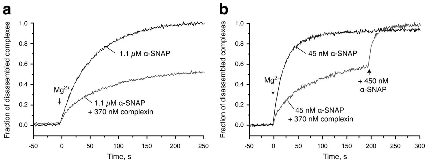
FIGURE 7. The SNARE complex-interacting protein complex 1 interferes more efficiently with disassembly in solution than on membranes. a , in solution, substoichiometric amounts of Cpx 1 reduced \alpha -SNAP efficiency during disassembly. Soluble, FRET-active complexes (Syb C28TR :SNAP25 C130TR :SyxH3, \sim 75 nm) were disassembled by 4.5 nM NSF with the help of 1.1 \mu M \alpha -SNAP in the presence or absence of 370 nM Cpx1. b , for the disassembly of membrane-inserted SNARE complexes, \sim 20 times less \alpha -SNAP was needed. Accordingly, 45 nM \alpha -SNAP was added to disassemble \sim 75 nm liposomal SNARE complex (SybTMR C28TR :SNAP25 C130TR :SyxH3). Addition of 370 nM Cpx 1 inhibited the reaction on membranes as well, but the inhibition could be overcome effortlessly when an additional 450 nM \alpha -SNAP was added (indicated by an arrow). Note that in this reaction, less than half the amount of \alpha -SNAP is present compared with the reaction shown in panel a . This corroborates the view that affinity of \alpha -SNAP to the SNARE bundle is augmented in the presence of the membrane.
