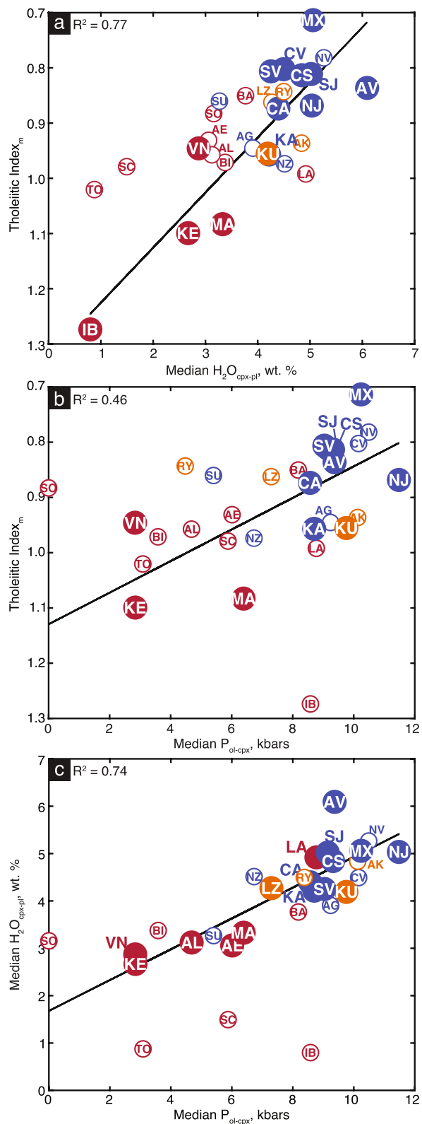
Figure 12. Correlations between the three liquid line of descent proxies. (a) Correlation between H 2 O cpx-pl proxy and THI m . (b) Correlation between P ol-cpx and THI m . (c) Correlation between H 2 O cpx-pl and P ol-cpx . Symbols and arc labels as in Figure 11. Arcs plotted with empty symbols with fewer than 15 samples are not included in linear fits.
