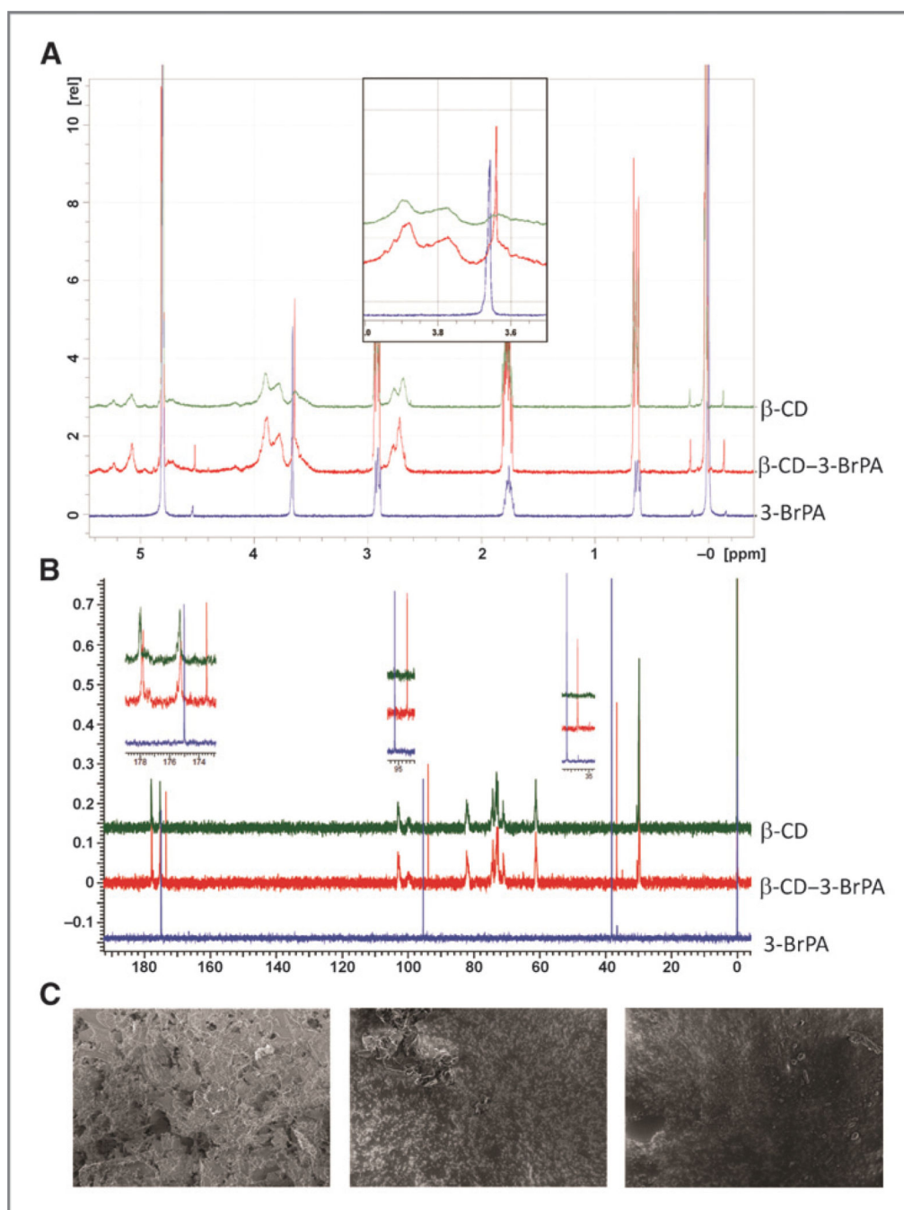
Figure 1. Characterization of microencapsulated 3-BrPA. A, ^1\text{H} NMR spectra of 3-BrPA (blue), \beta -CD-3-BrPA complex (red) and \beta -CD (green) in \text{D}_2\text{O} . The magnified insert highlights the methylene protons of 3-BrPA and upfield shift of the same methylene protons upon encapsulation of 3-BrPA in \beta -CD. B, ^{13}\text{C} NMR spectra of 3BrPA (blue), \beta -CD-3-BrPA complex (red), and \beta -CD (green) in \text{D}_2\text{O} . The inserts highlight an upfield shift of all 3 carbons of 3-BrPA upon complexation. C, SEM micrographs of 3BrPA (left), \beta -CD (center), and the \beta -CD-3-BrPA inclusion complex (right).
