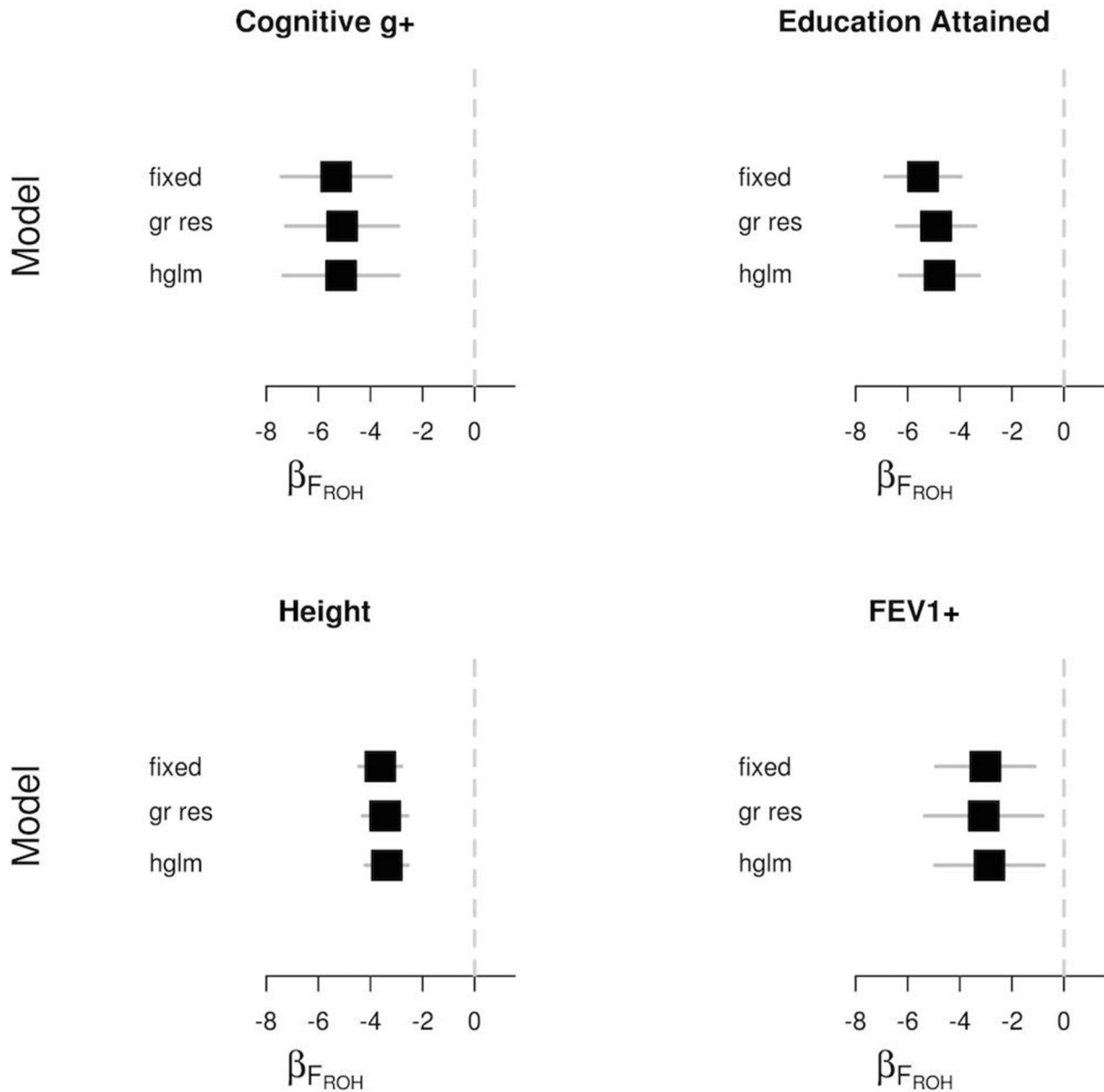
Extended Data Figure 6. Signals of directional dominance are robust to model choice Meta-analytical estimates of effect size and standard errors are plotted for various models. Fixed indicates no mixed modelling was used, gr res indicates the GRAMMAR+ residuals were fitted and hglm indicates the full hierarchical generalised linear mixed model was used. + indicates the phenotype was rank transformed; FEV1 is forced expiratory lung volume in one second; Cognitive g is the general cognitive factor. 15,355 subjects were used for cognitive g, 36,060 for educational attainment, 89,112 for height and 15,262 for FEV1.
