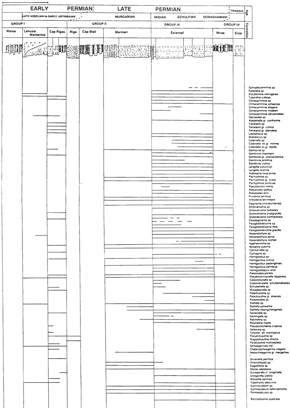
Fig. 3 Stratigraphic range of Permian Foraminifera and Algae in the Hydra Island. Same lithological section as Fig. 2
