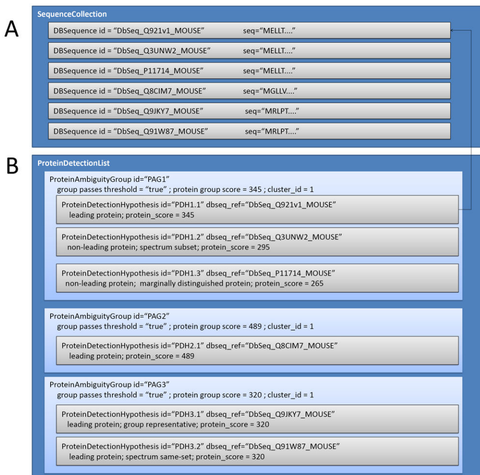
Figure 2. A and B. Graphical representation of how the concepts defined in Figure 1 map onto an mzIdentML file, following the recommendations presented in this manuscript. Each <ProteinDetectionHypothesis> has references back to all peptide spectrum matches (PSMs) on which the protein identifications are based (not shown – consult [19] for more details).
