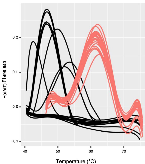
Fig. 3. L. pneumophila (red) showed a distinct melting temperature of 62°C, whereas Legionella spp. (black) showed either no melting curve or a melting temperature lower 55°C in melting curve analysis. (For interpretation of the references to colour in this figure legend, the reader is referred to the web version of this article.)
