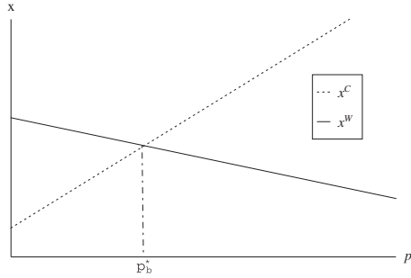
Figure 2. Implementation of the welfare-optimal level of riskiness.
