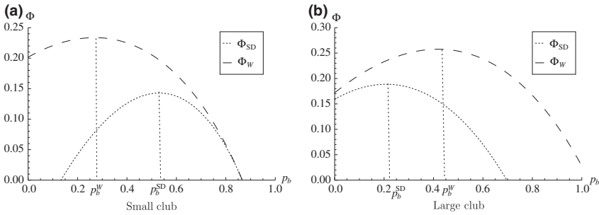
Figure 1. The objective function of the SD and the social planner for (a) small club and (b) large club.
