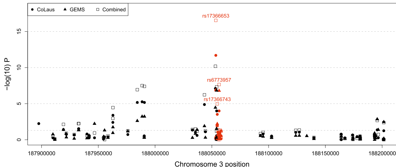
FIG. 1. Association analysis results based on joint analysis of GWAS and resequencing SNPs. The red and black symbols represent resequencing and GWAS SNPs, respectively.
