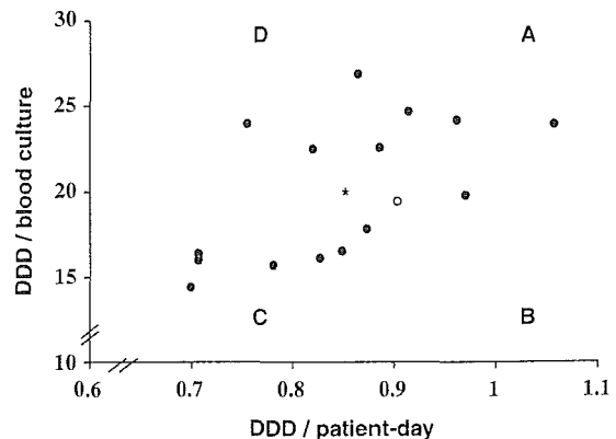
Fig. 1. Four-year quarterly use of antibiotics in a medical ward reported in defined daily doses (DDD) per patient-day ( x -axis) or per the number of blood samples drawn for culture ( y -axis). The line at one standard deviation above the mean on each axis divides the plot into four quadrants: quadrant A, high use on both scales; quadrant B, high use only when reported per patient-day; quadrant C, low use on both scales; quadrant D, high use only when reported per blood sample for culture. The open circle represents the reference trimester (see text). The star represents the mean use on both scales.
