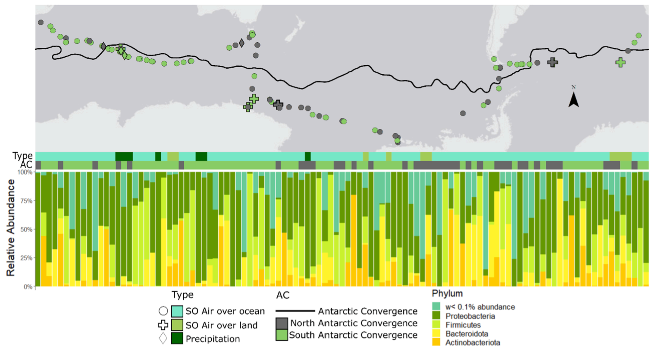
Fig. 1. Map of the air sampling locations, shaped by sample type and coloured by the origin of the air mass (back trajectory) relative to the Antarctic Convergence Zone. The relative abundance of bacterial taxa is given at the phylum level in the order of sampling. The microbial taxa dominating Southern Ocean (SO) air are highly variable with geographic location, even for consecutive samples and at the Phylum level.
