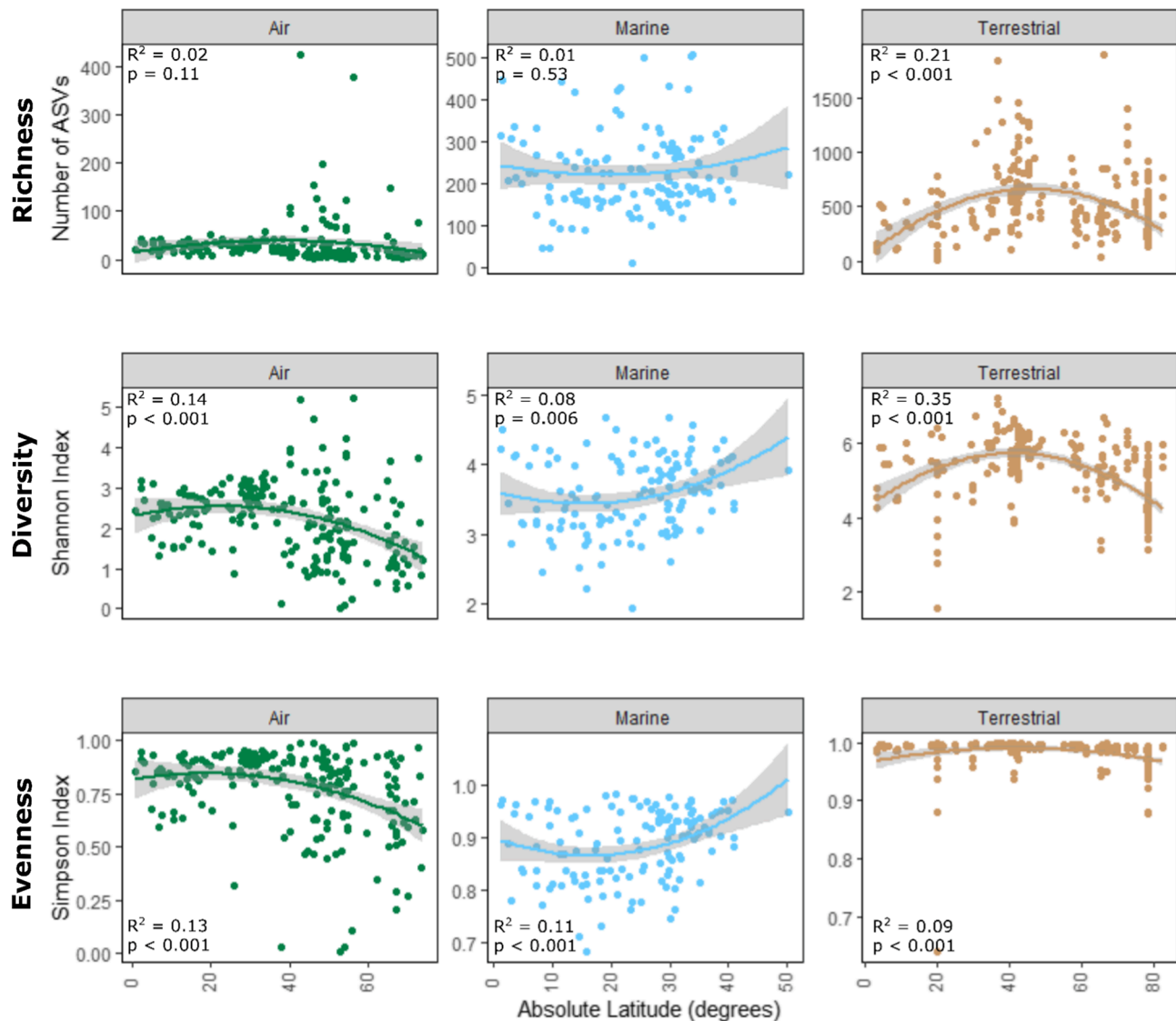
Fig. 3. Latitudinal distribution of the richness and diversity of air ( n = 198 ), marine ( n = 130 ) and soil ( n = 302 ) bacterial communities. The absolute latitude was used, merging northern and southern latitudes. The fits of second order polynomials are shown with R^2 and associated p-values.
