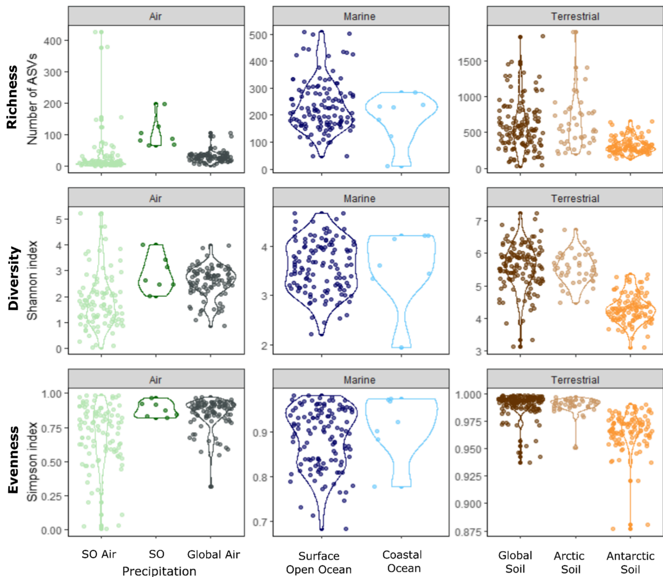
Fig. 2. Comparison of the alpha diversity of Southern Ocean air (SO Air, n = 100 ) and precipitation (SO Precipitation, n = 7 ) to other global air samples (global air, n = 98 ) and other non-air ecosystems including surface open ocean ( n = 123 ), surface coastal ocean ( n = 7 ), global soils ( n = 146 ), Arctic soils ( n = 43 ) and Antarctic soils ( n = 113 ).
