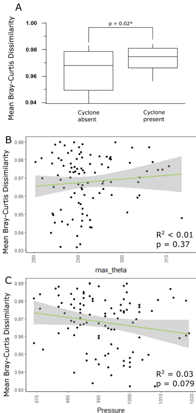
Fig. 6. A. Differences in community dissimilarity (Bray-Curtis) with the presence and absence of cyclones. B. Linear model of community dissimilarity (Bray-Curtis) along the maximum potential temperature of five-day back trajectories. C. Linear model of community dissimilarity (Bray-Curtis) along the pressure gradient.
