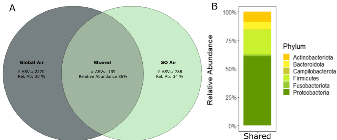
Fig. 5. A: number of ASVs (# ASVs) shared between global air and Southern Ocean air samples. The percentage indicates the relative abundance (Rel. Ab.) represented by the number of ASVs across all samples. B. Relative abundance of shared bacteria at the phylum level.
