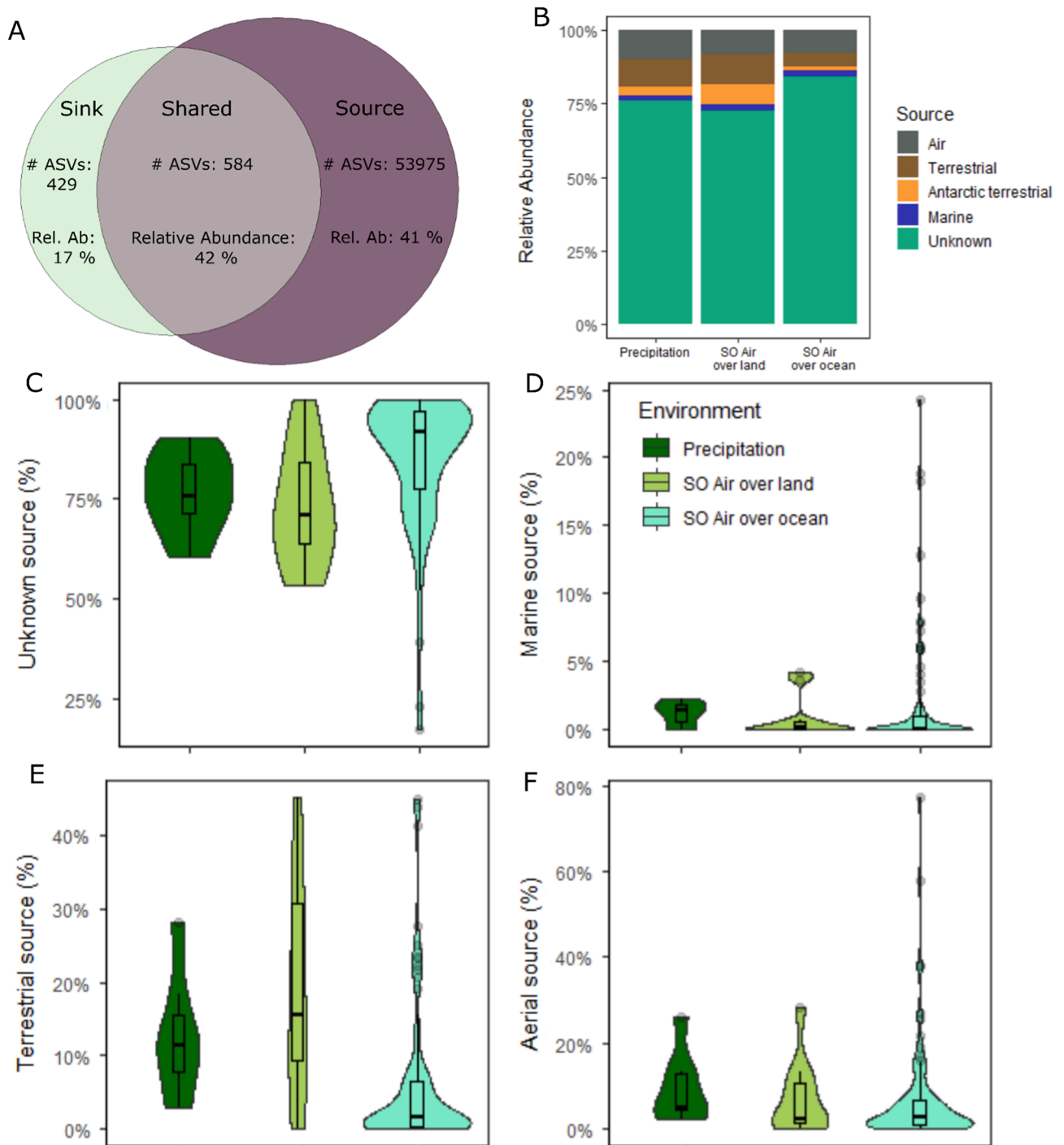
Fig. 7. A. Euler diagram showing the number of ASVs (# ASVs) with an origin identified from the global database and the relative abundance (Rel. Ab.). B. Mean potential origin of ASVs across each Southern Ocean sample type. C-F. Mean origin of ASVs per sample type.
