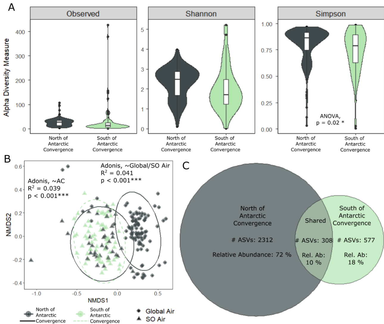
Fig. 8. Influence of the Antarctic Convergence Zone on microbial diversity above the Southern Ocean, using global air samples as well as the samples collected during the ACE expedition around the Southern Ocean. A. Alpha diversity comparisons B. NMDS of communities based on Bray-Curtis dissimilarity illustrating the differences between Southern Ocean air and Global air communities C. Euler diagram showing the number of shared ASVs north and south of the Antarctic Convergence Zone ASVs (# ASVs), weighted by the relative abundance (Rel. Ab.). of ASVs in percentages.
