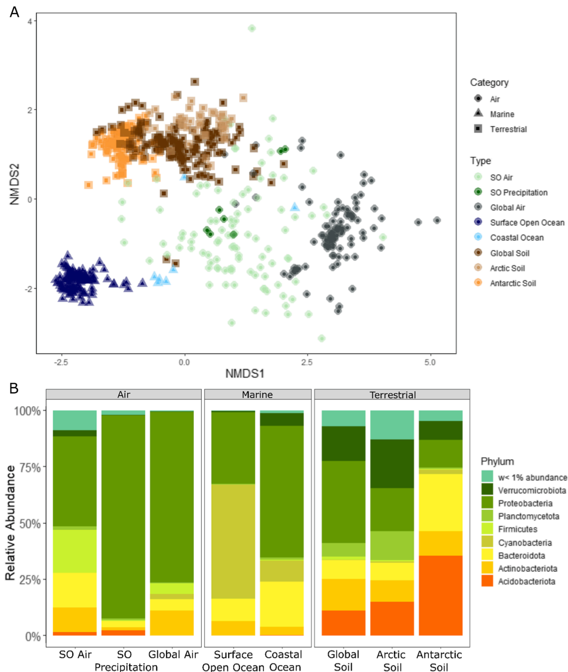
Fig. 4. A. Visualization of community dissimilarity using non-metric multidimensional scaling (NMDS) of the Bray-Curtis distance between air, marine, and soil bacterial communities. B. Relative abundance of bacteria at the phylum level.
