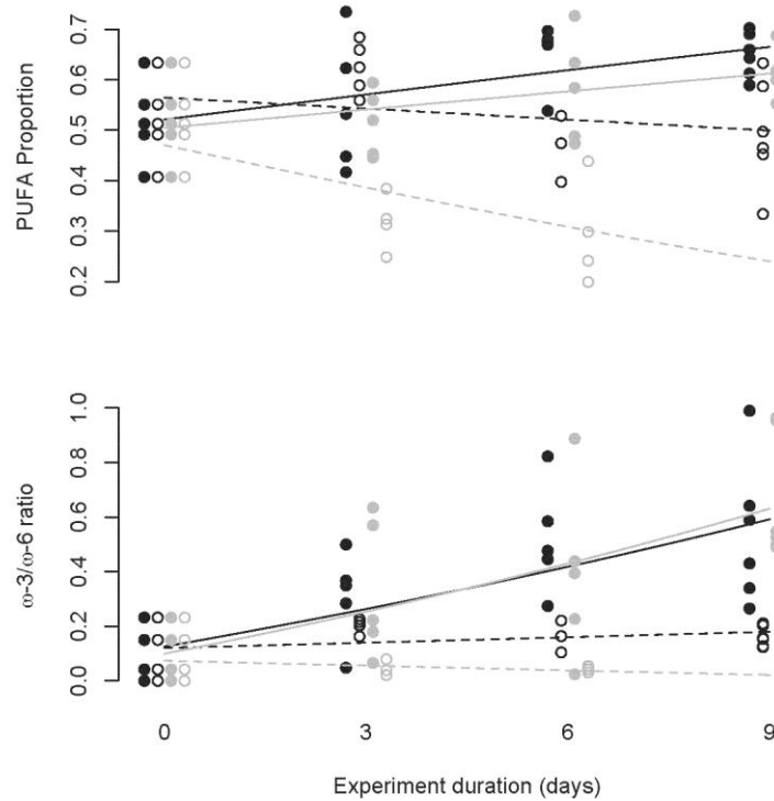
Figure 2. Modification of the larval PUFA proportion and the ω-3/ω-6 ratio during the experiment under various food treatments (A: black filled dots and solid lines, B: black empty dots and dashed lines, C: grey filled dots and solid lines, D: grey empty dots and dashed lines)
