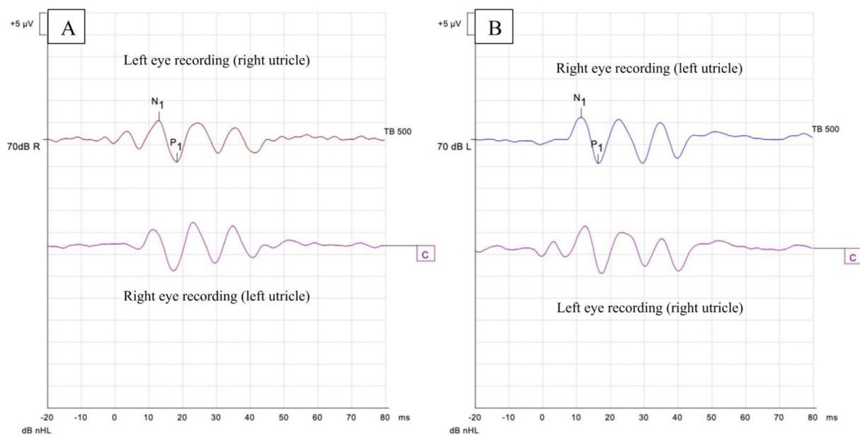
Fig. 1. Display of ocular vestibular evoked myogenic potentials (oVEMPs) recordings. A typical oVEMPs waves is displayed with N1 as the beginning of the excitation phase of the muscle and P1 as the beginning of the repolarization phase. On the left side (A), the upper wave represented the response of the right utricle measured below the left eye and the bottom wave represents the recording of the left utricle below the right eye at the same acquisition time. The right side (B) showed a second acquisition time where the left utricle was measured in the upper wave and the right utricle in the bottom wave. The Eclipse software allowed the data to be measured only in the superior waves of both sides (A and B), so two separate acquisitions were required to analyze both utricles.
