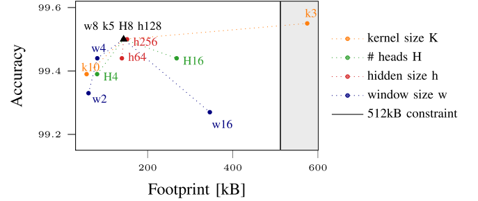
Fig. 2. Design points explored for EEGformer architecture definition. The selected point representing EEGformer is highlighted in black. The different curves represent the performance resulting from the selection of the parameters explored: window size, kernel size, number of heads, and hidden layer size. Shaded grey area: outside of the 512 kB feasibility region.
