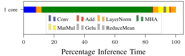
Fig. 6. Percentage inference time distribution for the different operators in EEGformer on GAP9 and 1 core execution.
