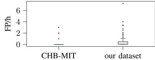
Fig. 3. Record-wise FP/h on the CHB-MIT dataset and our dataset with the EEGformer.
