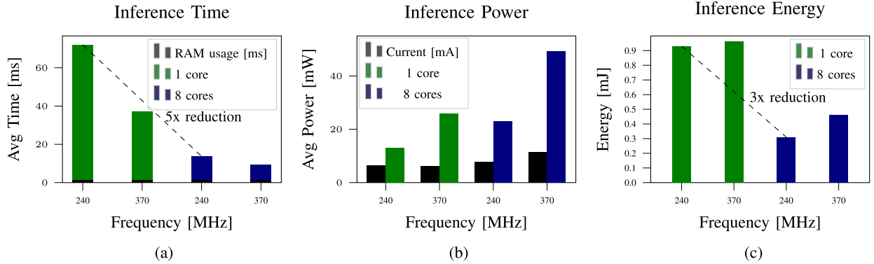
Fig. 5. Inference performance at different frequencies for single-core and multi-core execution on GAP9.
