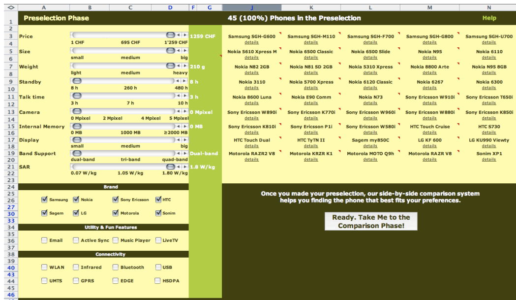
Figure 1: The pre-selection phase of ICA at the outset
