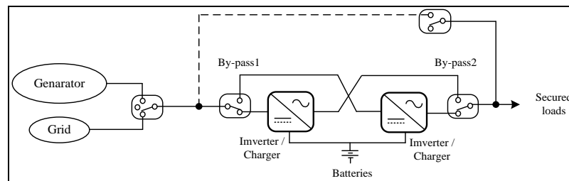
Figure 9 : Diagram of the proposed power backup and electricity stabilization
