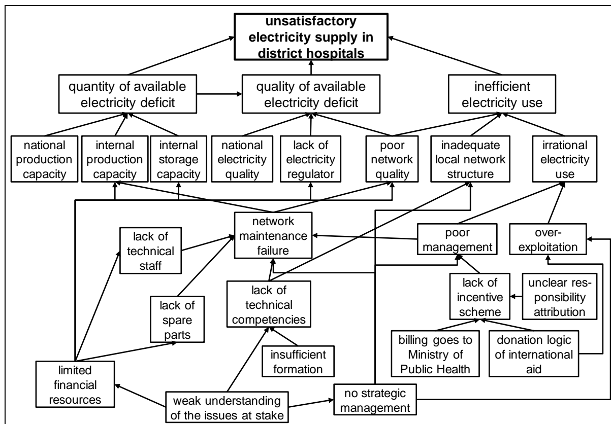
Figure 6 : Problem tree of the energy supply in district hospitals in Cameroon (bottom part)
