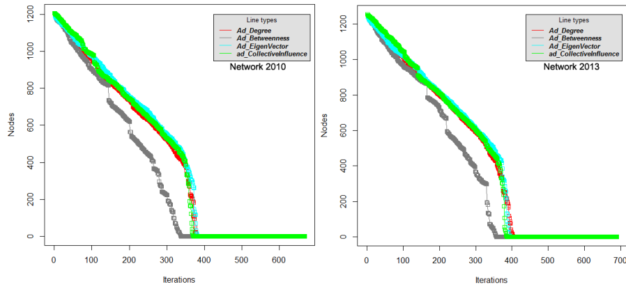
Fig. 3: Comparing the four best metrics to determine network connectivity. Adaptive Betweenness Centrality clearly outperforms other metrics as it is the quickest to disintegrate the entire network for both the years.
