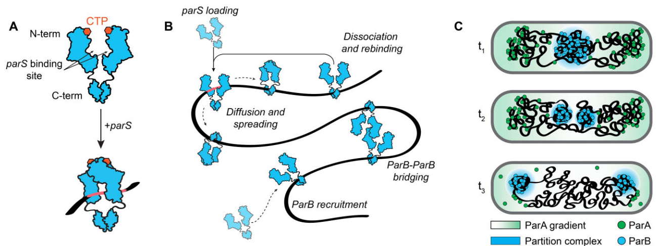
Figure 1. ParB binding to DNA and partition complex formation. (A) Schematic representation of ParB dimer structure and loading to DNA parS . Monomer units of ParB each bind a CTP nucleotide at their N-terminal domain (6). Upon recognition of parS site, ParB dimer undergoes a conformational change and forms a topological clamp around the DNA (11–13). (B) ParB loading, spreading and bridging on the DNA. Upon loading to the parS site (top left), ParB dimers lose the affinity to parS and start diffusing along the DNA (6,10). Upon CTP hydrolysis, ParB proteins either (i) dissociate from the DNA and recycle to parS (11), (ii) recruit a new ParB protein onto the DNA from the surrounding (44) or (iii) form a dynamic ParB–ParB bridge with another DNA-bound ParB dimer – which is essential for partition complex formation (14,17,24,41). (C) Schematic depicting directional movement of the partition complex in chromosome segregation. A large ParB partition complex is formed right after origin replication which contains nearly all cellular ParB proteins. The partition complex recruits SMC complexes (not shown in the schematic) that help to split two nascent origins (27,28). Nascent partition complexes interact with the nearby ParA molecules and start directionally moving towards the bacterial cell pole of the cell via diffusion ratchet mechanism (29–31).
