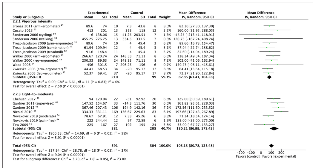
Figure 2. Pain-free walking distance (m) following vigorous and light-to-moderate exercise intensity. IV, inverse variance; SD: standard deviation of change.
