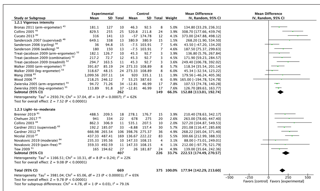
Figure 1. Maximal walking distance (m) following vigorous and light-to-moderate exercise intensity. IV, inverse variance; SD, standard deviation of change.
