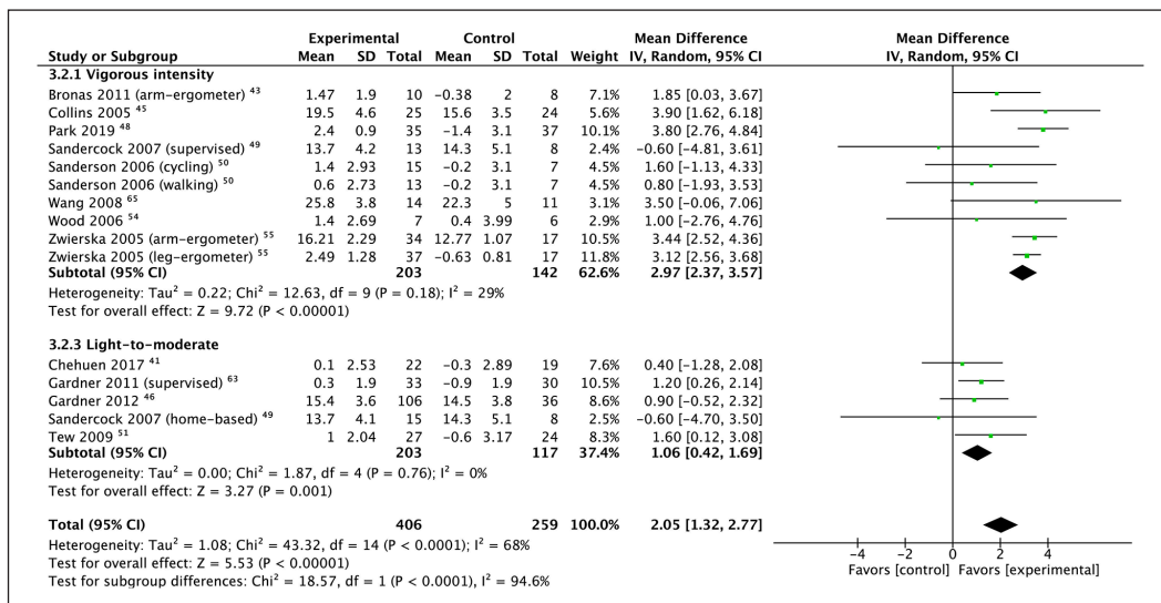
Figure 3. Cardiorespiratory fitness ( \dot{V}O_{2peak} , mL O 2 ·kg -1 ·min -1 ) following vigorous and light-to-moderate exercise intensity. IV, inverse variance; SD, standard deviation of change.
