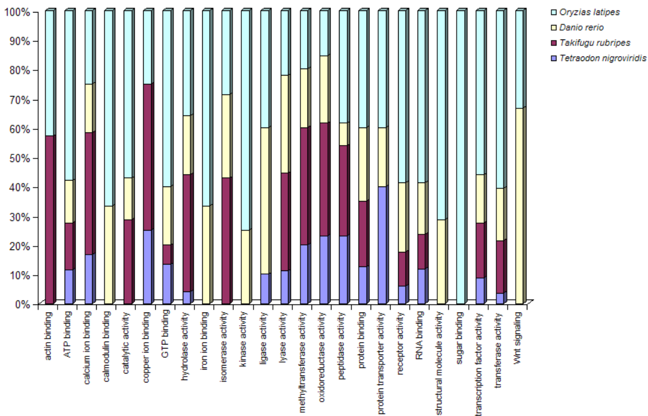
Figure 6 Comparison of rates of gene functions (according to GO) of all fish protein genes with significantly lower distance to the human ortholog than other fish species.
