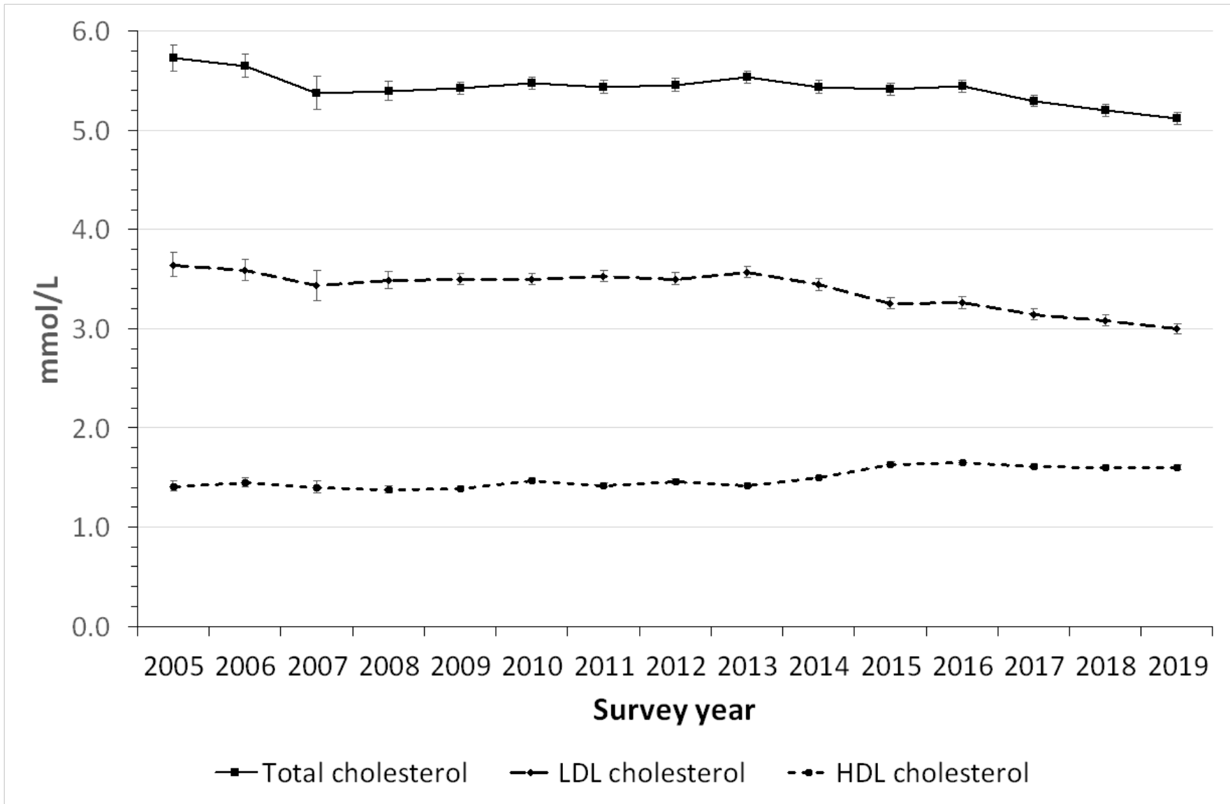
Supplementary figure 1: trends in total, LDL and HDL cholesterol between 2005 and 2019, Bus Santé study, Geneva, Switzerland. Results are expressed as multivariate-adjusted mean and 95% confidence interval. All trends are significant at p < 0.001 .
