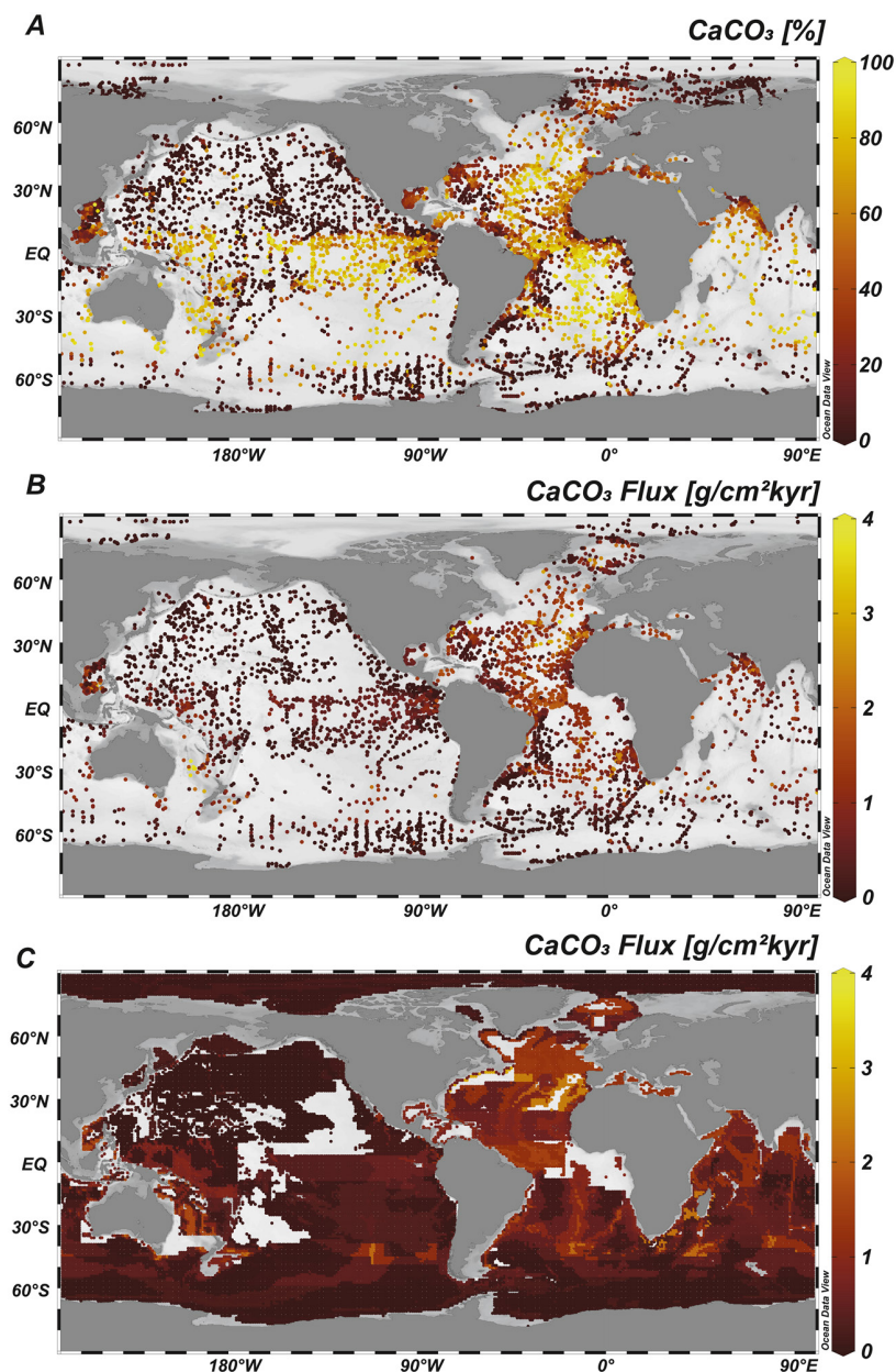
Figure 2. (a) Weight percentage of \text{CaCO}_3 , (b) flux of \text{CaCO}_3 in surface sediments using spatially-interpolated Th-normalized fluxes with discrete \text{CaCO}_3\% observations, and (c) flux of \text{CaCO}_3 using spatially-interpolated Th-normalized fluxes and spatially-interpolated \text{CaCO}_3\% values. Uncolored (white/gray) zones are shallower than 1 km or zones that do not contain any Th-normalized flux observations.
