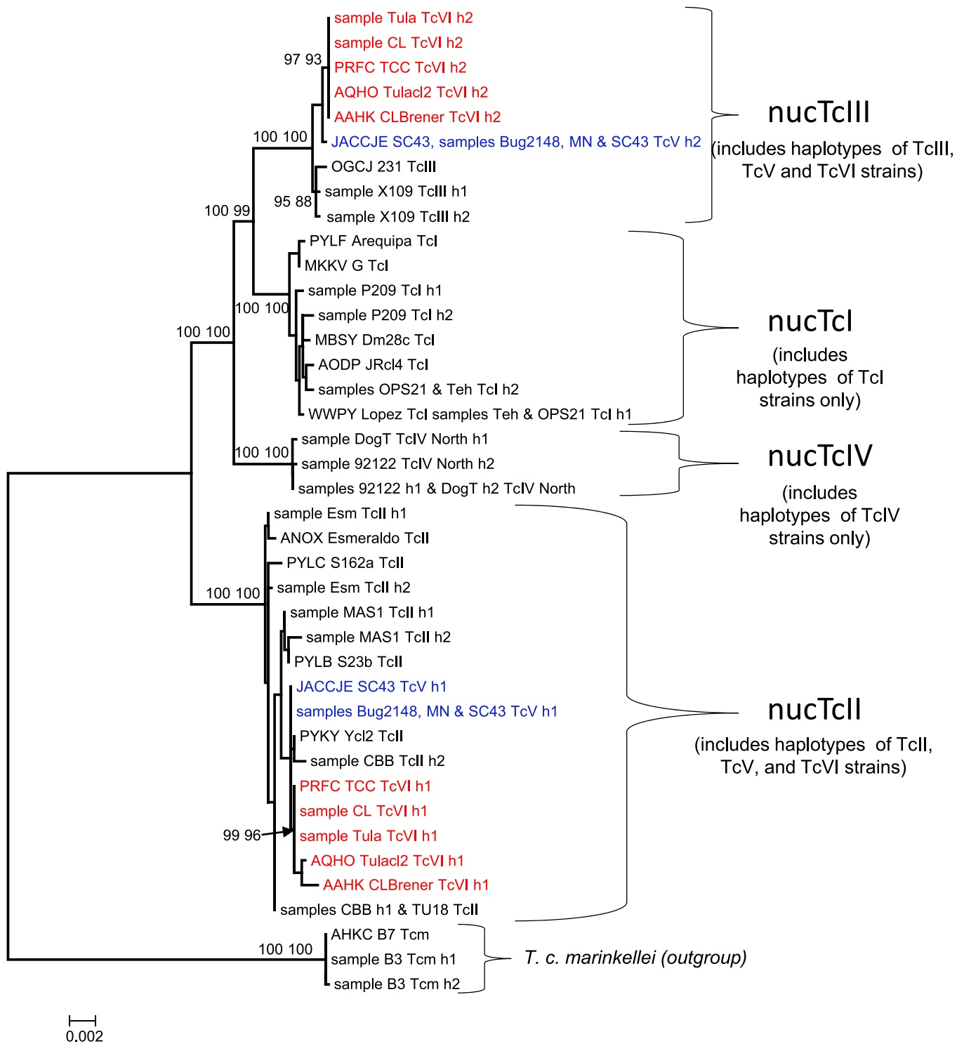
Fig. 2. Maximum likelihood (ML) tree of the 40 different haplotypes (3959 nucleotide positions, see alignment in File S2 (B)) resulting from, the concatenation of nine single-copy nuclear gene fragments ( DHFR-TS , GPI , GPX , HMGAR , AP , PDK , RB , RHO1 , and TR ) for 31 strains: 16 presently sequenced by NGS sequencing (leaf name beginning by “sample”) and from BLAST hits against 15 WGS assemblies of Trypanosoma cruzi . The numbers at the nodes are 1) the posterior probability of the Bayesian analysis, and 2) the bootstrap value for the ML tree. The terms h1, 2, 3, ...n correspond to the different haplotypes for a specific sample, if any.
