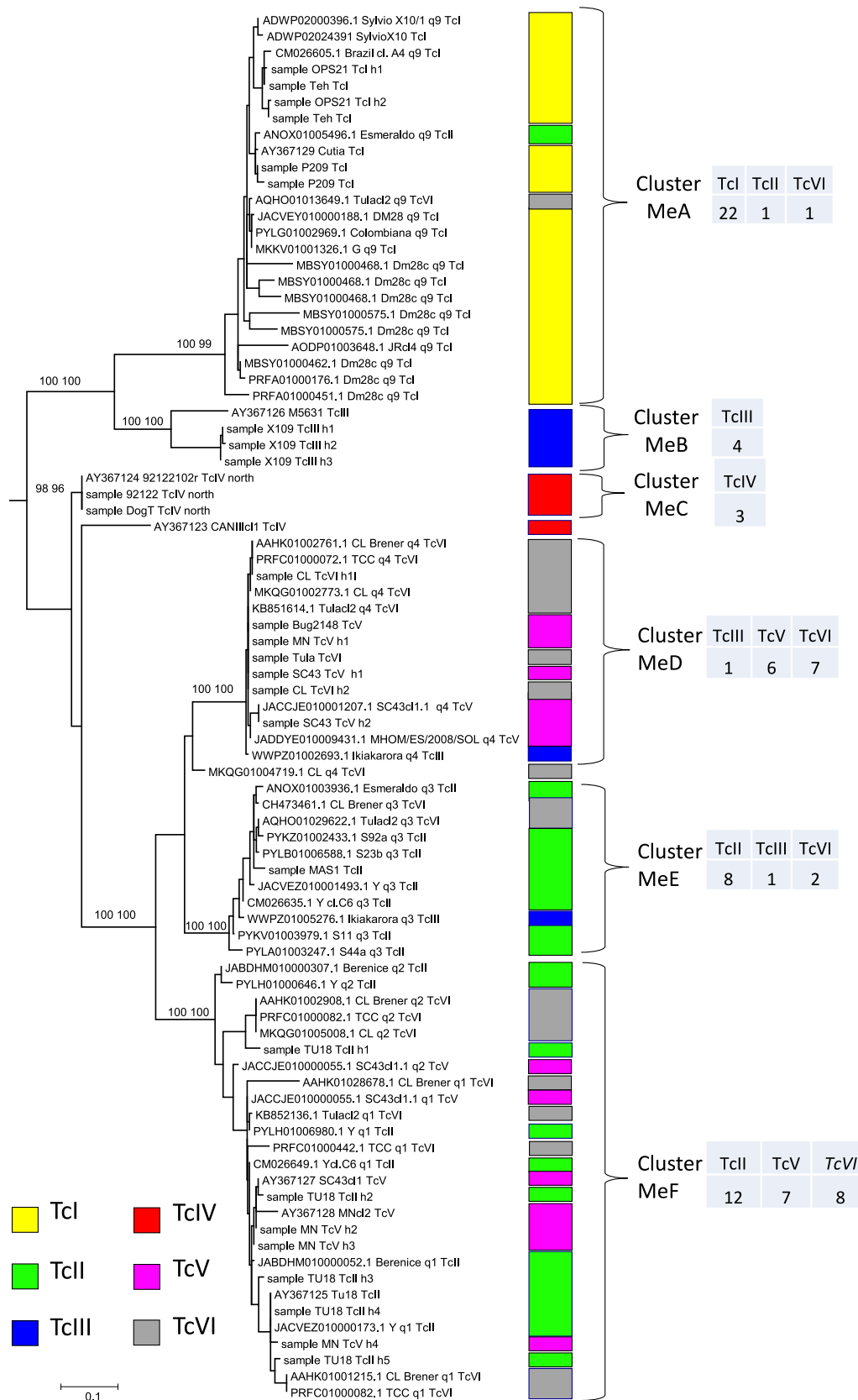
Fig. 3. Maximum likelihood (ML) tree involving 85 mini-exon intergenic sequences coming from our NGS sequencing (leaf names beginning by “sample”), from BLAST hits against the 36 WGS of Trypanosoma cruzi , and seven informative mini-exon sequences from the nucleotide NCBI database, including sequences from TcIII and TcIV which are drastically under-represented in the WGS. See alignment in File S2 (C). The numbers at the nodes are 1) the posterior probability of the Bayesian analysis, and 2) the bootstrap value for the ML tree. The terms q1, 2, 3,..0.9 in sequence names refer to the best query hits obtained with BLASTn using the corresponding nine mini-exon reference sequences (File S1). The terms h1, 2, 3, ...n correspond to the different haplotypes for a specific sample, if any.
