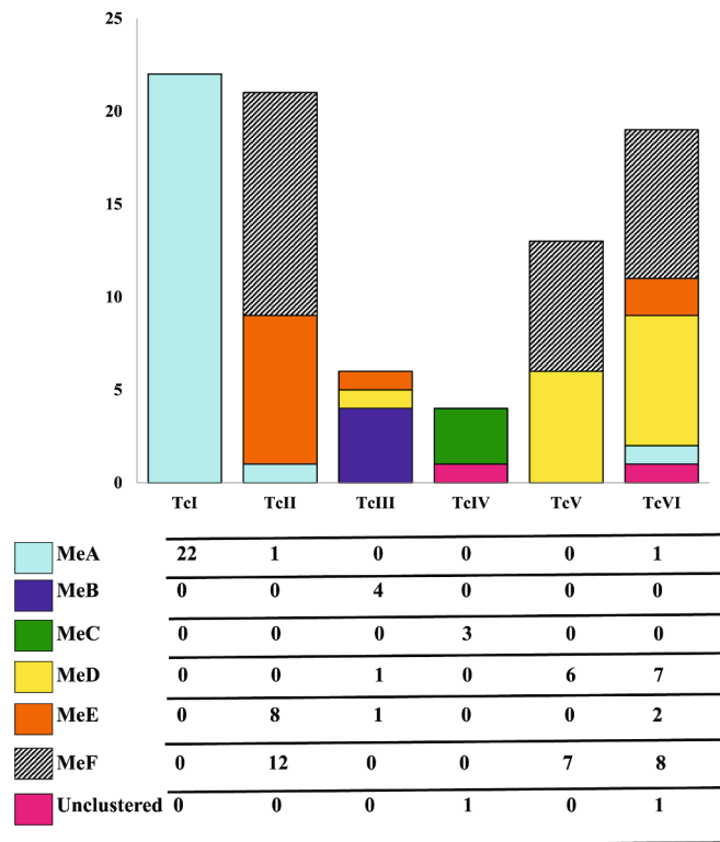
Fig. 4. Distribution of the 85 haplotypes of mini-exon intergenic sequences through the six clusters (A to F) obtained on the corresponding clustering tree (see Fig. 3) and the six DTUs of Trypanosoma cruzi (TcI to TcVI). Note that only haplotypes from TcI and TcIV were present in a single mini-exon cluster, (MeA and MeC, respectively); all haplotypes from other DTUs were present in two or more mini-exon clusters.
