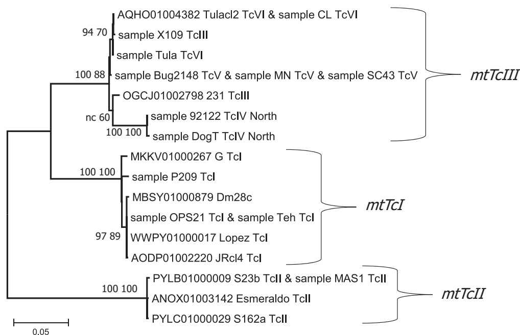
Fig. 1. Maximum likelihood (ML) tree of the 16 different haplotypes (on 1274 nucleotide positions, see alignment in File S2 (A)) of T. cruzi resulting from the concatenation of three mitochondrial gene fragments COII , CytB , and ND1 , and coming from 21 DNA sequences in total: 12 obtained by NGS sequencing of our samples (leaf name beginning by “sample”) and nine from BLAST hits against WGS assemblies of Trypanosoma cruzi . The numbers at the nodes are 1) the posterior probability of the Bayesian analysis, and 2) the bootstrap value for the ML tree; “nc” (not clustered) indicates that this particular cluster was absent in the analysis with the corresponding method.
