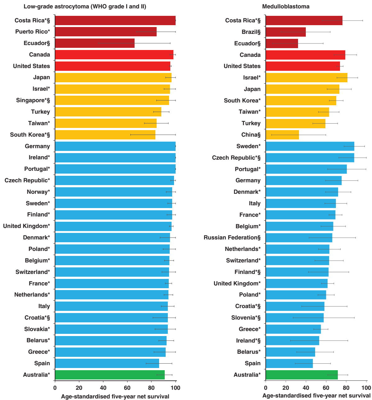
Fig. 1. Age-standardized 5-year net survival (%) with 95% confidence interval, by country: children (0–14 years) diagnosed with low-grade astrocytoma or medulloblastoma during 2010–2014. *Countries with 100% coverage of the national population. §Survival estimates not age-standardized. Continents are identified by different colors. In each panel, countries are ranked from highest to lowest, based on survival during 2010–2014.
