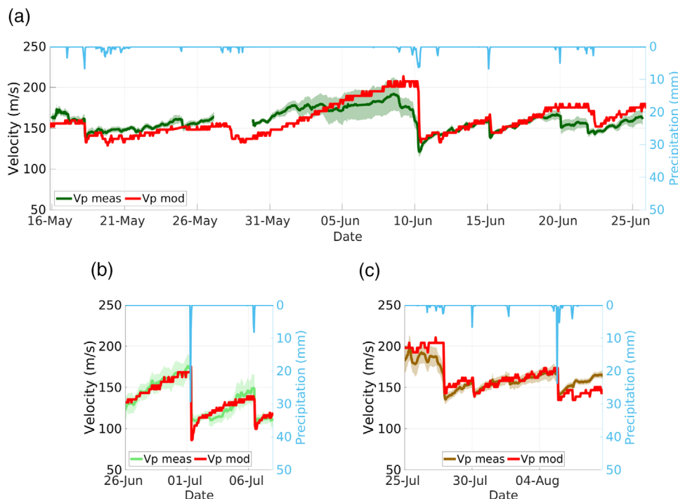
FIGURE 5 Time-series of modeled (mod) and measured (meas) P-wave velocities ( V_p ) for (a) compacted ley, (b) noncompactd ley, and (c) compacted bare soil along with precipitation data (light blue right hand axes)
