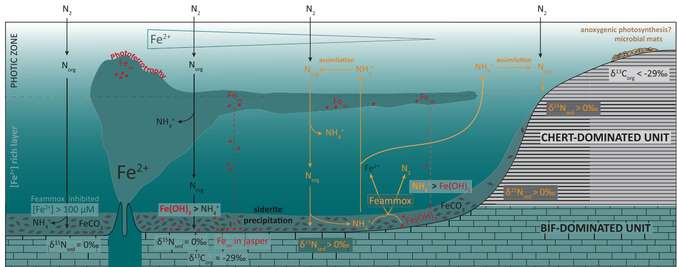
FIGURE 4 Schematic model illustrating how the iron and nitrogen cycles could have interacted in an anoxic and ferruginous Archean ocean, as recorded in the BRC formation. Following the sedimentary model described by Tice and Lowe (2004), the chert-dominated unit is related to platform settings and gives way to the BIF-dominated unit as depth increases toward basin settings. The water column is chemostratified, with a lower \text{Fe}^{2+} -rich layer supplied by hydrothermal iron fluxes. Siderite precipitates either at the chemocline or in the sediment and accumulates on the seafloor, forming the BIF-dominated unit. The abundance of siderite follows a gradient away from the hydrothermal discharge zones. In the absence of free \text{O}_2 in the water column, iron oxides observed in the BRC jasper layers can be produced through photoferrotrophy when dissolved \text{Fe}^{2+} reaches the photic zone. Organic nitrogen is sourced to the water column by diazotrophic \text{N}_2 fixation and is either consumed by organisms or ammonified as \text{NH}_4^+ . In the chert-dominated unit, iron oxides are scarce and therefore quantitatively consumed by Feammox. The residual ammonium becomes enriched in ^{15}\text{N} and can carry this enrichment to organic matter when reassimilated, which would produce positive sedimentary \delta^{15}\text{N} values. In the iron-rich settings of the BIF-dominated unit, \delta^{15}\text{N} values are close to 0\text{‰} , recording only biological \text{N}_2 fixation by diazotrophs. This could either result from quantitative consumption of \text{NH}_4^+ by Feammox due to an excess of iron oxides or to an inhibition of Feammox by dissolved \text{Fe}^{2+} concentrations exceeding 100\ \mu\text{M} .
