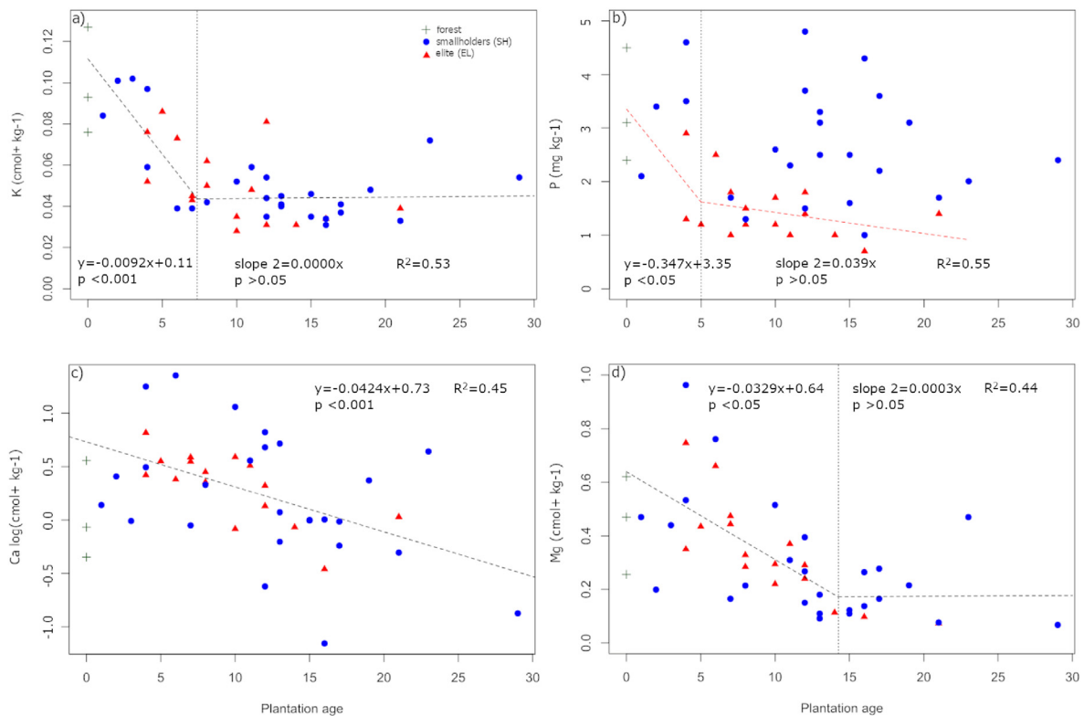
Fig. 3. Available nutrient content in the topsoil (0–10 cm) depending on farming system and age for available K (a), P (b), Ca (c) and Mg (d). Dashed lines represent the regression or segmented regression between nutrient content and age, regardless of the farming system when this factor was not significant (a, c and d) or only in elite plantations when an interaction between factors occurred (b). Vertical dotted line represents the breaking point of the segmented regression.
