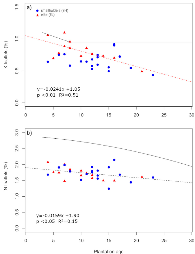
Fig. 4. Oil palm leaflets contents of a) K and b) N in function of plantation age and farming system. Solid lines represent the critical K and N contents in function of age, estimated by Rafflegeau et al. (2010) from industrial plantations in the study region. Dashed lines represent the effect of age regardless of the farming system (b) or only in elite plantations (a).
