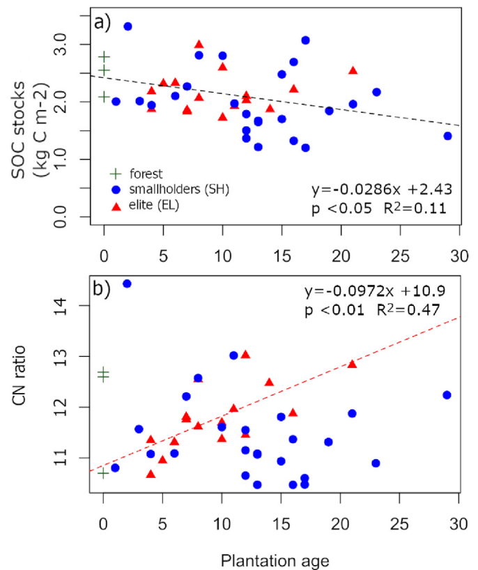
Fig. 2. Effect of forest conversion to oil palm plantations on a) soil organic carbon (SOC) and b) C:N ratio, depending on age and farming system. Dashed lines represent in a) the effect of age regardless of farming system as it had no effect on SOC, and in b) the effect of age on C:N ratio only in elite plantations as the effect in smallholder plantations was not significant.
