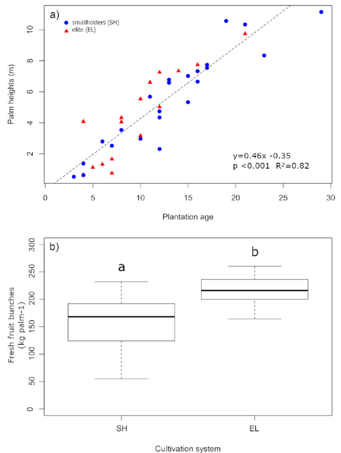
Fig. 5. Effect of farming system on biomass productivity indicated by (a) palm height and (b) fresh fruit bunches (FFB) weight per palm. Dashed lines in (a) represent the effect of age regardless of the farming system. Lowercase letters in (b) represent significant difference between boxplots.
