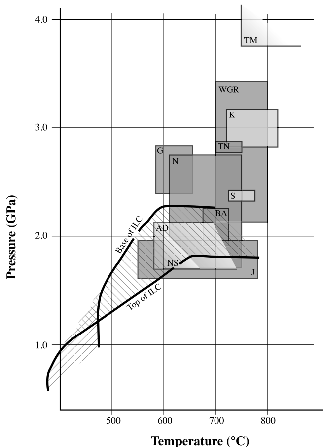
Figure 2. Pressure-temperature estimates for peak conditions of the different eclogite occurrences in Himalayas (light gray) and Scandinavian Caledonides (dark gray) compared with the pressure-temperature distribution in the Indian Lower Crust from India toward Tibet deduced from thermokinematic modeling [Hetényi et al. , 2007]. TM, Tso Morari; K, Kaghan; S, Stak; AD, Ama Drime; NS, North Sikkim; WGR, Western Gneiss Region; TN, Tromsø nappe; G, Garborg; N, Norrbotten; BA, Bergen Arc; J, Jämtland. References are as in Table 1.
