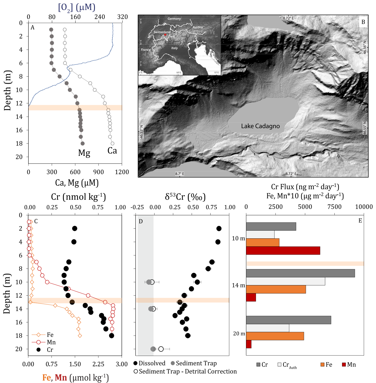
Figure 1. Water column data. (a): [O_2] , [Ca] and [Mg] . (b): map showing the location of Lake Cadagno. (c): dissolved [Cr] , [Fe] and [Mn] . (d): dissolved and sediment trap \delta^{53}Cr (uncorrected and corrected for detrital chromium (Cr), see Section S.5 in Supporting Information S1). (e): Sediment trap Cr, Fe and Mn fluxes (note different depth range). The orange box in (a and c–e) indicates the chemocline. The gray box in (d) indicates average detrital \delta^{53}Cr (Schoenberg et al., 2008).
