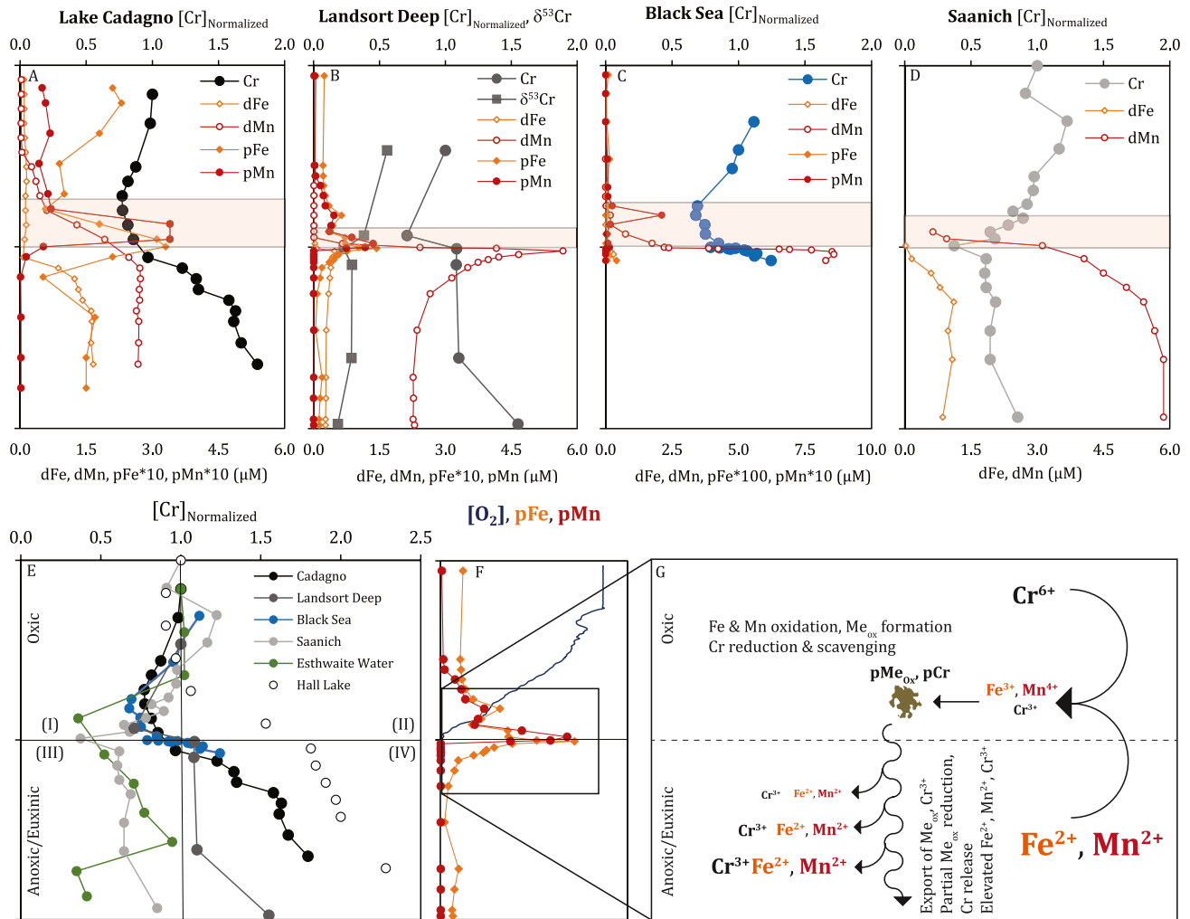
Figure 3. Compilation of anoxic basin data with conceptual mechanistic diagram. Chromium, Fe (orange) and Mn (red) concentrations in the dissolved (open circles, dFe and dMn) and particulate (filled circles, pFe and pMn) phases from Lake Cadagno (a), black, this study, pFe and pMn: Ellwood et al., 2019), Landsort Deep (b), dark gray, this study), the Black Sea (c), blue, Cr: Mugo, 1997, Fe and Mn: Lewis & Landing, 1991), and Saanich Inlet (d), Emerson et al., 1979, light gray, only dissolved data). (e) combines (a–d) with Esthwaite Water (green, Achterberg et al., 1997) and Hall Lake (white, Balistrieri et al., 1994). In (a)–(f), the y-axis ranges from the surface to sediments, with the chemocline at the center. In (a)–(f), [Cr] is normalized to surface concentrations. The orange shading in (a–d) indicates the zone of enhanced Fe and Mn redox cycling above the chemocline. (f–g) show a schematic of metal cycling in this zone, using Landsort Deep data (f) (see Table S8 in Supporting Information S1).
