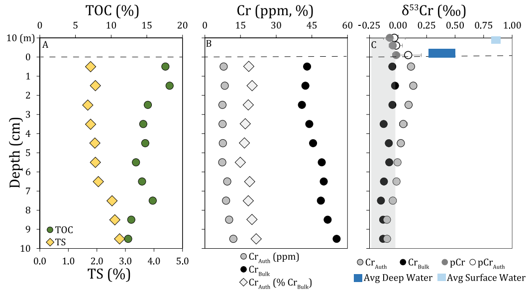
Figure 2. Near-surface sediment data. (a): bulk sediment parameters (TOC, TS). (b): near-total digest ( Cr_{Bulk} ) and leach ( Cr_{Auth} ) concentrations, and Cr_{Auth} as % Cr_{Bulk} . (c): \delta^{53}Cr_{Bulk} and \delta^{53}Cr_{Auth} with average surface and deep water dissolved \delta^{53}Cr and sediment trap \delta^{53}Cr (total and detrital-corrected), along with average detrital \delta^{53}Cr (gray box).
