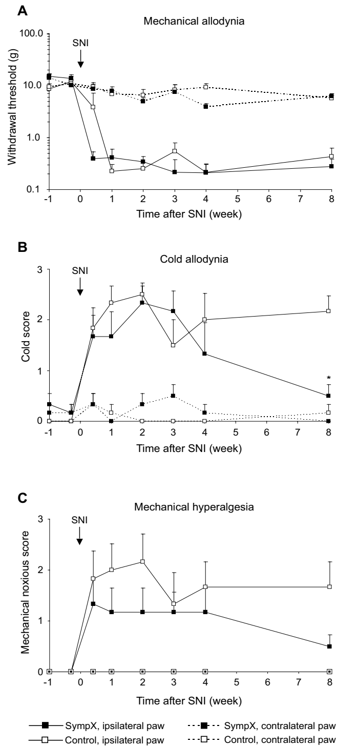
Figure 2 Effect of chemical sympathectomy on the development of neuropathic pain-related behavior induced by SNI. A. Paw withdrawal thresholds to mechanical stimuli using a calibrated series of von Frey hairs were not different between chemically sympathectomized group (sympX, n = 6) and vehicle treated group (control, n = 6) before and after SNI. B. Response to cold using an acetone drop was similar before SNI in both groups. No overall effect was demonstrated, except at the latest time point studied (* p < 0.01 ). C. Mechanical hyperalgesia evoked by pin prick showed no difference between groups.
