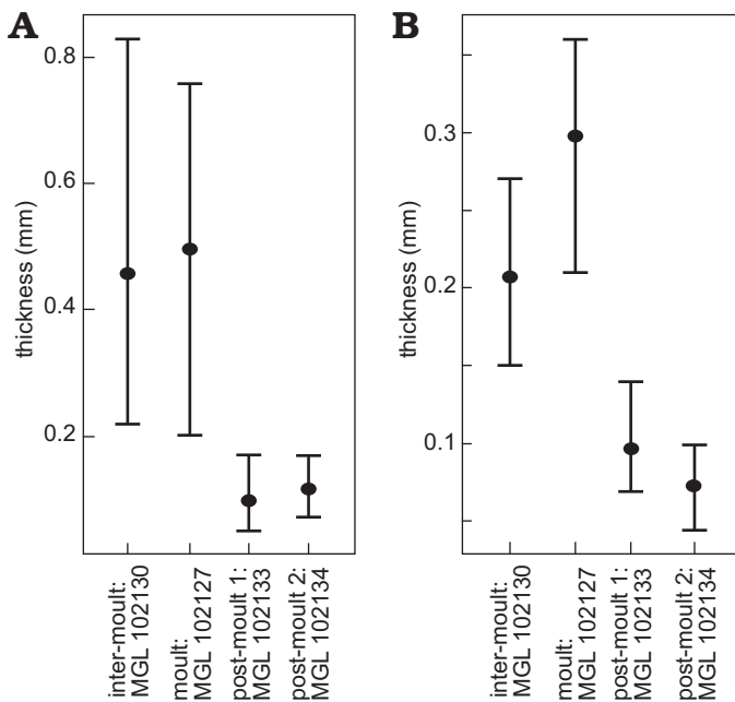
Fig. 4. Graphs showing means (points) and ranges of exoskeleton thickness for cephalae (A) and thoraces (B) of the thin sectioned trilobites Symphysurus ebbestadi .
