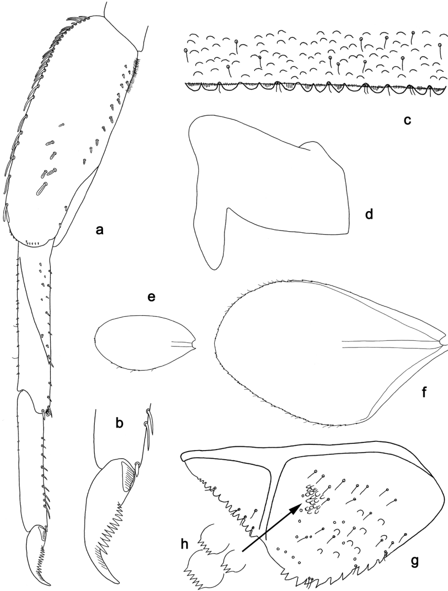
Figure 3. Tenuibaetis fujitanii sp. n., larva morphology: a Foreleg b Fore claw c Tergum IV d Left side of metanotum e Gill I f Gill IV g Paraproct, arrow: notched scales h Notched scales on paraplect. e and f at same scale.
