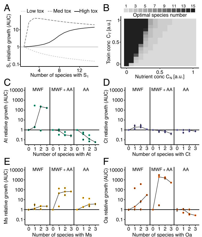
Fig. 4. (A) Our model predicts that, for a focal strain S_1 , an increasing community size eventually becomes detrimental. The number at which such competition starts depends on environmental toxicity. (B) The optimal number of species with respect to the AUC of a focal strain (peak in A) varies with nutrient and toxin concentrations. (C–F) Each species' growth expressed in fold change in its AUC divided by its mean monoculture AUC in the 3 different media. Each point shows the mean of a culture treatment composed of 1 to 4 species, and vertical black lines show standard deviations. Black lines connect the median points. In environments where a species could not grow alone, the curves are hump-shaped, while, in more benign environments, species grow less well in the presence of others.
