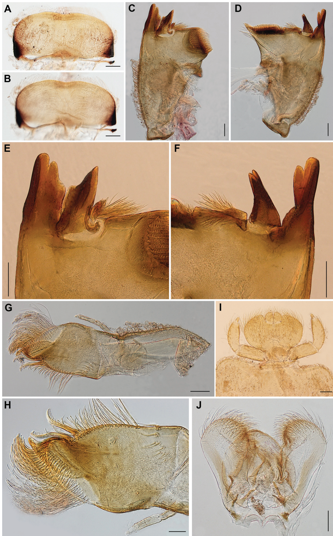
Figure 2. Cincticostella tornata : A dorsal view of labrum; B ventral view of labrum; C left mandible; D right mandible; E left mandibular canine; F right mandibular canine; G maxilla; H crown of maxilla; I labium; J hypopharynx. Scale bars: 0.1 mm (A–D, G–I, J); 0.05 mm (E, F, H).
