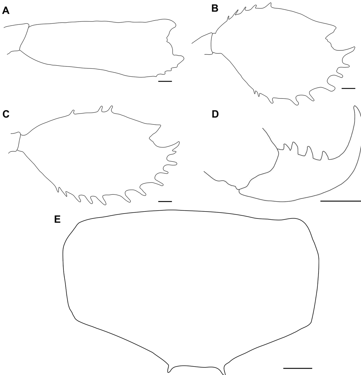
Figure 4. Cincticostella tornata : A forefemur; B mid femur; C hind femur; D forefemur claw; E tergite X. Scale bars: 0.2 mm (A–C); 0.1 mm (D, E).
