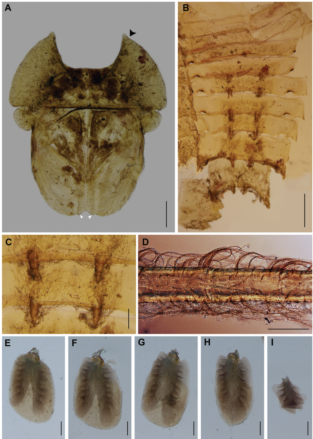
Figure 3. Cincticostella tornata : A thorax (black arrow tip: concave apical margin of prothorax; white arrow tips: small pair of triangular protuberances between forewing pads); B abdomen; C tergites VI–VII; D cercus; E–I gills of segments III–VII respectively. Scale bars: 1 mm (A, B); 0.25 mm (C–I).
