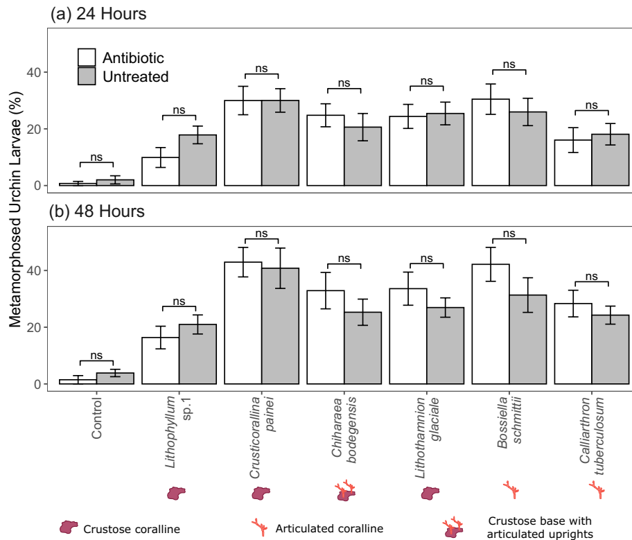
FIGURE 4 Mean ( \pm SE) percentage of red sea urchin ( Mesocentrotus franciscanus ) larvae metamorphosed on different crustose and articulated coralline algal species with their microbiome reduced (Antibiotic) and those with their natural microbiome (Untreated) after (a) 24 and (b) 48 h. Paired t -test results (corrected with Bonferroni correction for multiple comparisons) shown for each coralline algal species. ns=not significant ( p > 0.05 ). See Table 1a for sample sizes. [Color figure can be viewed at wileyonlinelibrary.com ]
