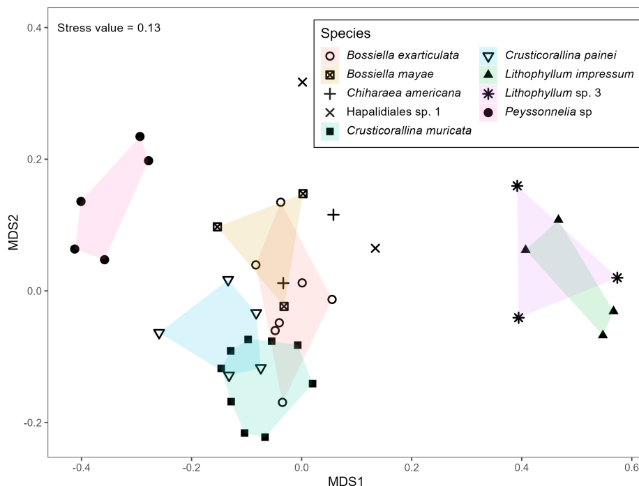
FIGURE 2 Non-metric multidimensional scaling (nMDS) ordination plot showing microbiome community composition on different coralline algal species and fleshy red algal crusts ( Peyssonnelia sp.) with shapes linking samples from the same species when the sample size is greater than two. [Color figure can be viewed at wileyonlinelibrary.com ]
