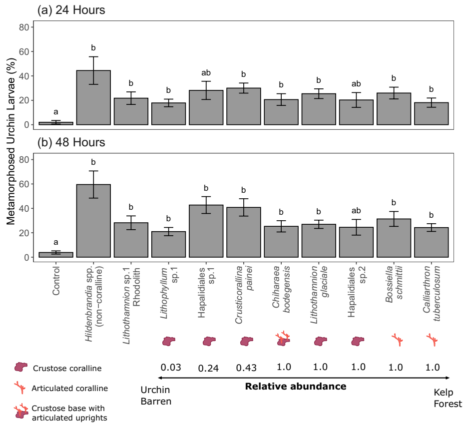
FIGURE 3 Mean ( \pm SE) percentage of red sea urchin ( Mesocentrotus franciscanus ) larvae that underwent metamorphosis on different coralline algal species after (a) 24 and (b) 48 h. Different letters above bars indicate significant differences (Tukey's test, p < 0.05 ). The relative abundance of each coralline algal species in kelp forest compared with urchin barren habitat is shown and is based off data collected by Hind et al. (2019). The relative abundance of the fleshy red Hildenbrandia spp. was 0.83 in kelp forests compared with urchin barrens. Lithothamnion sp.1 rhodolith is a free-living crustose coralline algae observed on soft sediment habitat and therefore does not have an associated relative abundance. See Table 1a for sample sizes. [Color figure can be viewed at wileyonlinelibrary.com ]
