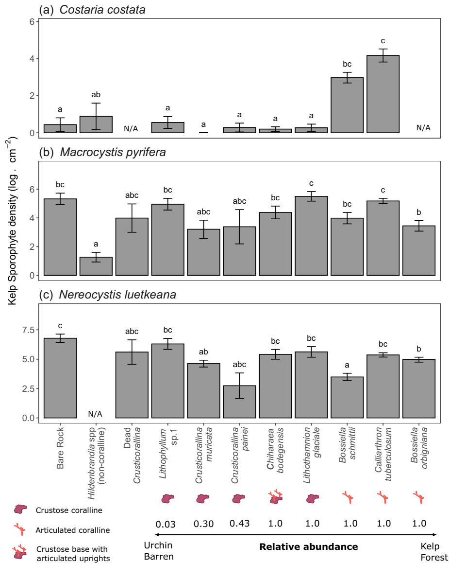
FIGURE 5 Mean juvenile sporophyte ( \pm SE) density of (a) Costaria costata , (b) Macrocyctis pyrifera , and (c) Nereocystis luetkeana juvenile sporophytes on different coralline algal species. Shown on a log scale to better visualize differences. Different letters above bars indicate significant differences (Tukey's test, p < 0.05). The relative abundance of each coralline algal species in kelp forest compared with urchin barren habitat is shown and is based off data collected by Hind et al. (2019). The relative abundance of the fleshy red Hildenbrandia spp. was 0.83 in kelp forests compared with urchin barrens. See Table 1b for sample sizes. [Color figure can be viewed at wileyonlinelibrary.com ]
