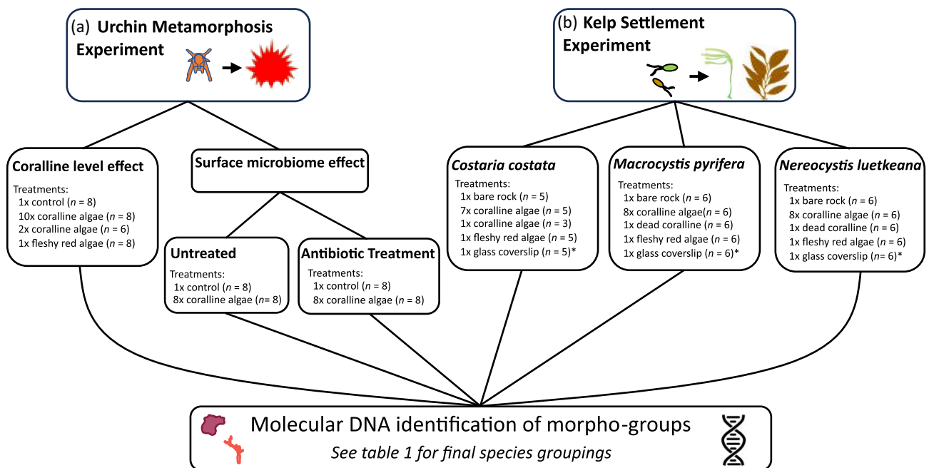
FIGURE 1 Schematic diagram of the experimental design used in manipulations of coralline algae to test (a) urchin metamorphosis and (b) kelp settlement. Treatments are given as number of groups/morpho-groups and the number of replicates ( n ). *Glass cover slips were used to track changes in kelp gametophyte/sporophyte development and not used in analysis. [Color figure can be viewed at wileyonlinelibrary.com ]
