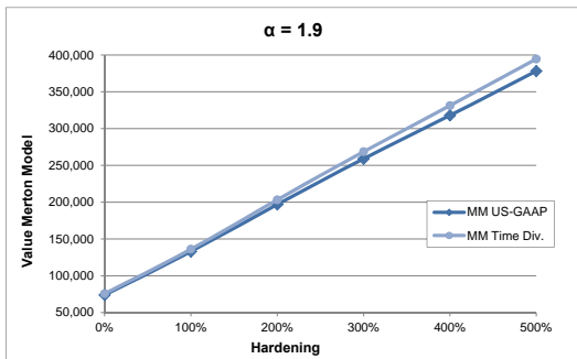
Figure 6: Value of the call option under a hardening of the market cycle for Fréchet losses.
