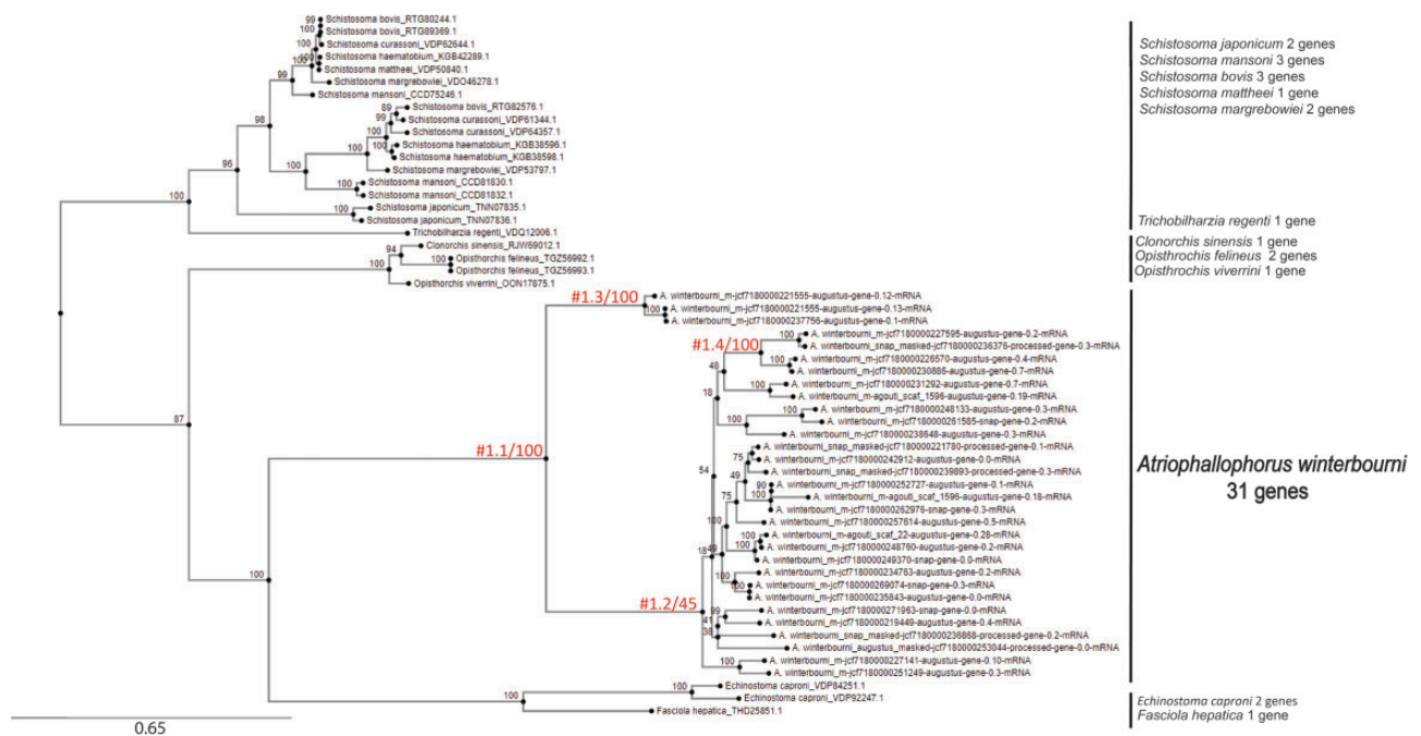
Fig. 4. —Gene tree of gene family HOG 25969 created with IQ-TREE. The tree is unrooted. Each name is a species name followed by the original gene name (protein name). Atriofallophorus winterbourni gene names are shortened version of gene names in supplementary table S10, Supplementary Material online. The numbers above branches indicate ultrafast bootstrap support, for the #1 branches the bootstrap support is after a backslash. The branches labelled with #1.X indicate the separation between the foreground branches and the background branches (distinction used in codeml for investigation of selection). The test for selection compares the dN/dS between the foreground branch and the background branches. The total number of genes in this HOG per trematode species is given next to each species name.
