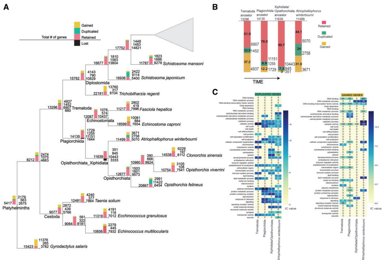
FIG. 3. —(A) Number of duplicated, retained (1:1 orthologs) and gained genes resulting after each point of speciation obtained from the analysis of HOG in pyHam, mapped onto a phylogenetic tree of trematodes (for original, see supplementary fig. S6, Supplementary Material online). The total number of genes at each point is indicated on the left-hand side of the bar and the total number of retained (pink), duplicated (green), and gained (yellow) genes are indicated on the right-hand side of the bar. The bars indicate the proportions of genes in each category. The lost genes are indicated only for the three ancestral genomes: the Trematoda ancestor, the Plagiorchida ancestor, and the Opisthorchiata/Xiphidiata ancestor. (B) The proportions (on the bars) and the total numbers (next to the bars) of retained (pink), duplicated (green), and gained (yellow) genes in each reconstructed ancestral genome leading to A. winterbourni . The oldest ancestral genome is on the left-hand side and the extant A. winterbourni genome on the right-hand side. The total number of genes per genome is above each bar beneath the name. (C) Heatmaps summarising the GO enrichment analysis of the duplicated and gained genes in the three reconstructed ancestral genomes and the extant genome of A. winterbourni . All enriched GO terms were categorized into GO slims, listed on the y-axis of each heatmap. The colors indicate the mean IC value of each GO slim category and the number printed on top is the number of unique genes within that GO slim category (see Materials and Methods).
