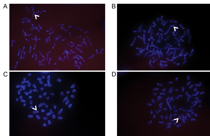
Figure 4: Clones derived from plasmid transfection have single genomic integration sites.
