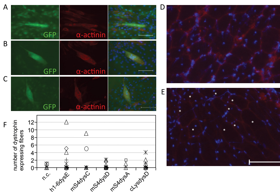
Figure 5: Differentiation and in vivo dystrophin expression from transfected mesoangioblast stable cell clones.
