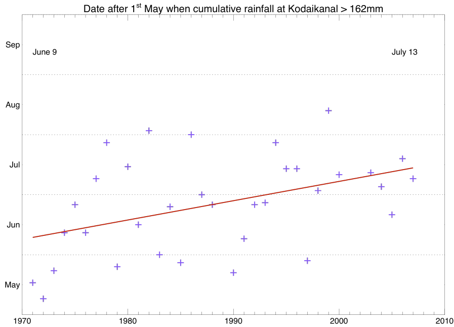
Fig. 5 Start dates (blue crosses) between 1971 and 2007 of the onset of the SW monsoon at Kodaikanal using the definition described in the text. The line of best fit is significant at the 5% level. The dates on the graph indicate the start and end dates of the line of best fit.
