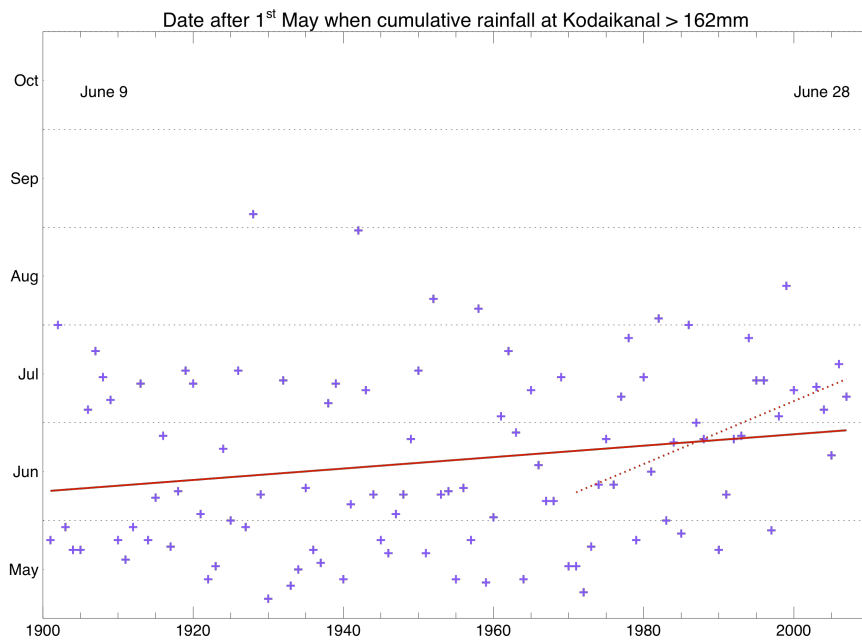
Fig. 6 As Figure 5 but for the period 1901 to 2007 using combined data from Bryant Park and Kodaikanal Observatory. The dashed red line represents the line of best fit between 1971 and 2007.
