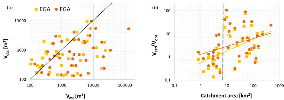
Figure 9. (a) Modelled LW V_{est} (large scenario) versus observed wood volume V_{obs} during past events. The black line shows the line of equality (1 : 1 line). (b) Ratio of V_{est}/V_{obs} versus catchment area.
