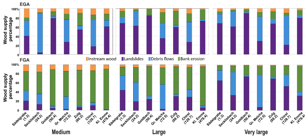
Figure 8. Percentage of wood volume supplied by each process, model, and scenario for selected studied sites; the names and catchment area (km 2 ) are provided in the abscissa.
