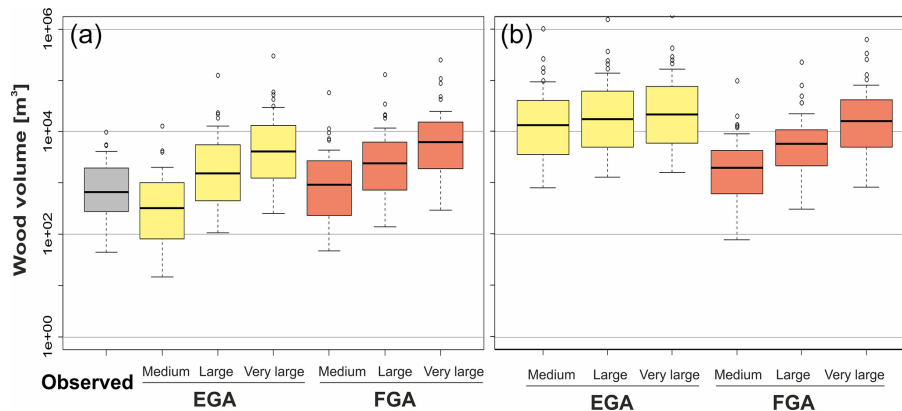
Figure 5. Boxplots of wood supply (a) and potential (b) volume ( m^3 ) estimated by the two models EGA and FGA and the three scenarios (i.e. medium, large, very large). “Observed” refers to the reported LW volumes after flood events ( n = 40 ; shown in grey colour), in most cases equivalent to the large scenario.
