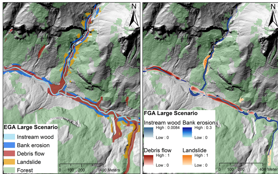
Figure 4. Large-scenario comparison of model outputs from the EGA (left) and FGA (right) at the Spiggebach torrent within the Chiene river catchment (canton of Bern). Potential recruitment areas are shown for landslides (orange), debris flows (red), and bank erosion (dark blue). The stream network (light blue) also includes instream wood loads. Background: digital terrain model (hillshade), © swisstopo.
