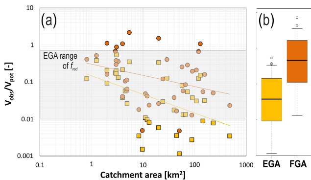
Figure 10. Ratio of observed wood volumes and potential wood volumes computed by the two models for all sites and their catchment areas. The grey rectangle shows the reduction factor range used for EGA computations.
