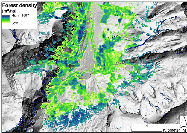
Figure 2. Example of the wood stock raster map in the Grosse Melchaa catchment near Stöckalp (canton of Obwalden). Background: digital terrain model (hillshade), © swisstopo.
