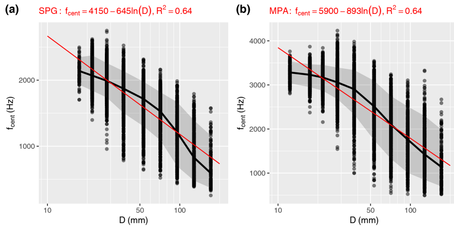
Figure 10. Oberrach flume site. Centroid frequency f_{\text{cent}} vs. grain size D for packets with the five largest amplitudes per experimental run vs. grain size D . Only single grain size class experiments were used. (a) For the SPG system, (b) for the MPA system.
