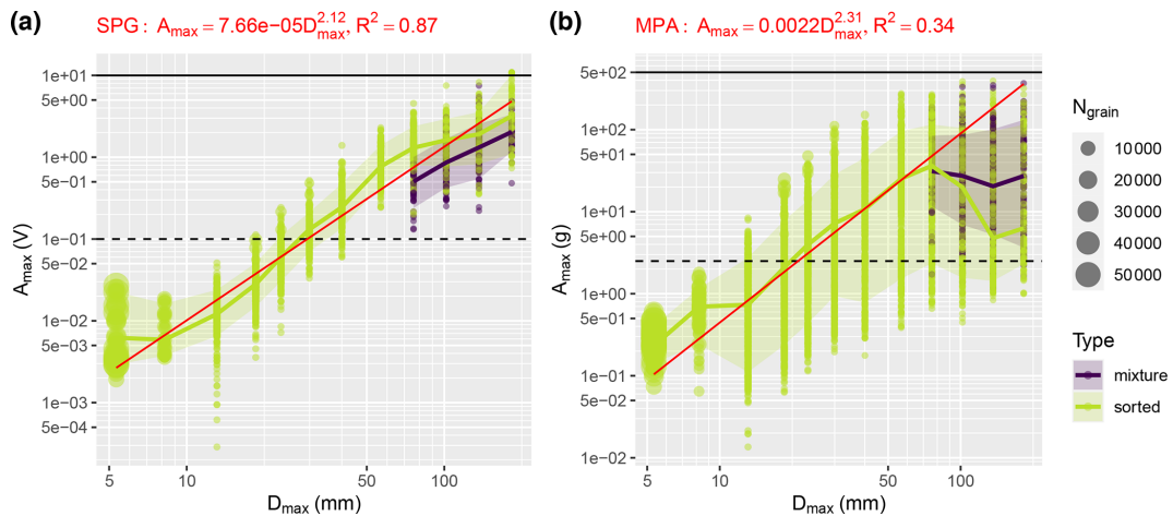
Figure 9. Oberrach flume site. Maximum (positive) amplitude A_{max} recorded per experimental run vs. grain size D . The power-law regressions are based on the sorted (single grain size class) experiments only. (a) For the SPG system, (b) for the MPA system.
