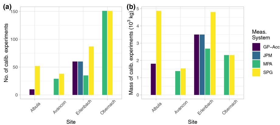
Figure 3. Amount of calibration data in terms of (a) number and (b) total sampled mass with direct measurement methods at the different sites and for different measurement systems. At the Avançon de Nant, some calibration experiments included very high transport rates of fine grains (potential shield or cover effect on the plates), and those were removed for further analysis (Nicollier et al., 2022b; Antoniazza et al., 2022).
