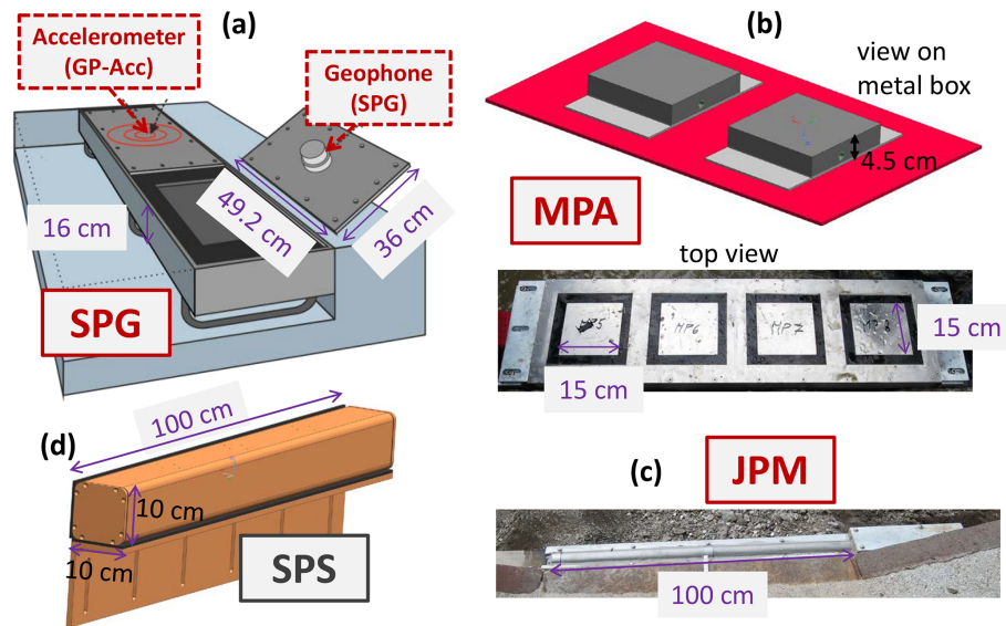
Figure 2. Sketches with the main dimensions of the four systems. For (a) the SPG and (b) the MPA, the plate thickness is 15 and 8 mm, respectively. For (c) the JPM, the pipe diameter is 48 mm, and its wall thickness is 3 mm. The (d) SPS is a new prototype system (with preliminary test results), and the wall thickness of the square steel pipe is 8 mm.
