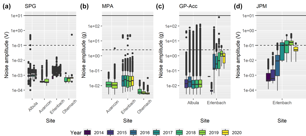
Figure 4. Background noise level of SPG (a), MPA (b), GP-Acc (c), and JPM (d) for each year at different sites during non-transport conditions. For the field sites, the noise levels (amplitudes) were derived from the IQA values. For the Obernach site, the noise levels were determined as the median absolute amplitudes of the raw signal of each experiment. The dashed and solid lines indicate the threshold for impulse counts ( A_{\min} ) and the upper limit of the output range, respectively.
