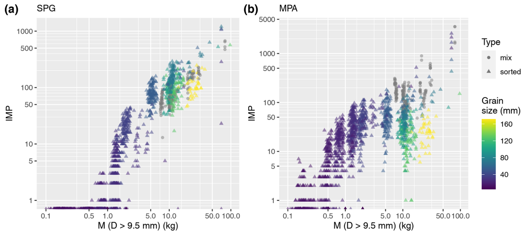
Figure 8. Oberrach flume site. (a) SPG impulses and (b) MPA impulses vs. total transported mass M , for both flume experiments with single grain size classes (“sorted”) and those with mixed grain sizes (“mix”). The size class indicates the median grain size present in each experiment.
