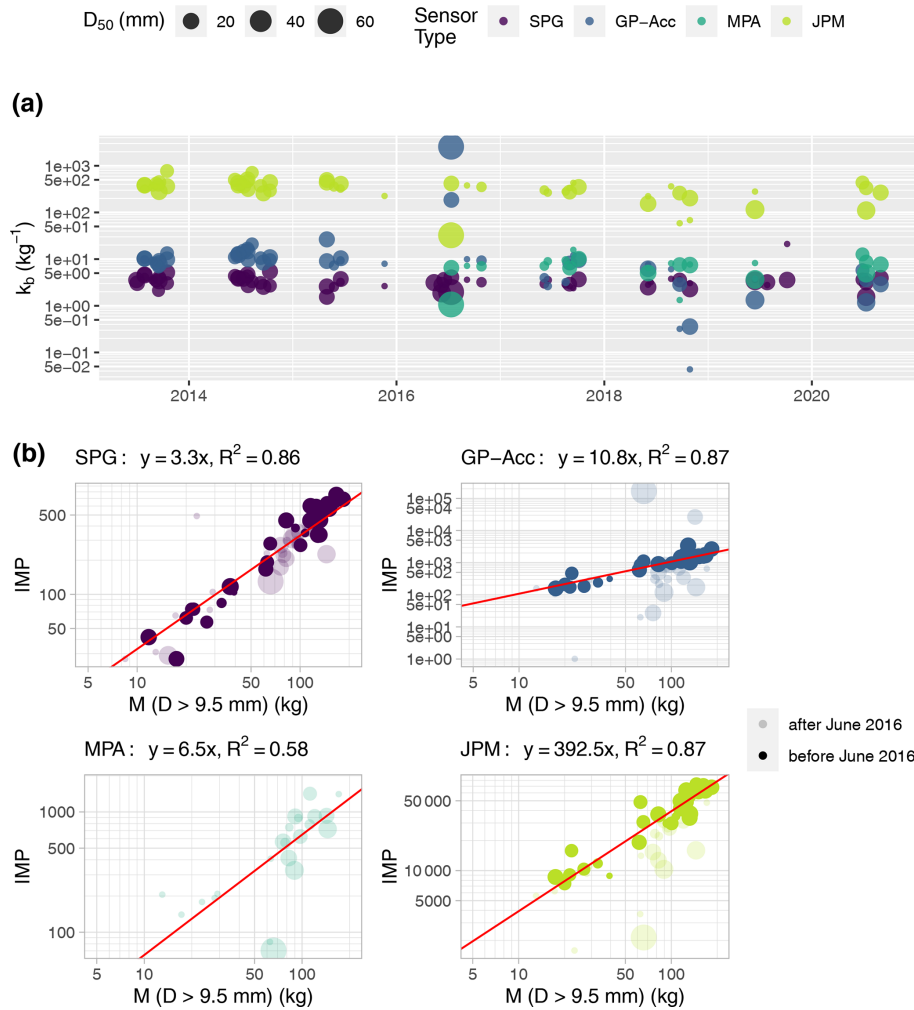
Figure 5. Calibration measurements at the Erlenbach. (a) Temporal evolution of ratio of impulses per transported mass k_b . (b) Calibration relation for each measurement system, showing the IMP vs. bedload mass M . Samples lighter than 5 kg were excluded, and only grains with D > 9.5 mm were retained from the direct samples. In June 2016, the data acquisition system recording the signal of the GP-Acc and the JPM systems was changed; the same acquisition system was used to record the MPA measurements (starting in 2016). For the GP-Acc and the JPM, regression equations refer only to the period before June 2016. The SPG measurements were recorded by a different system, which did not change in the period 2013 to 2020.
