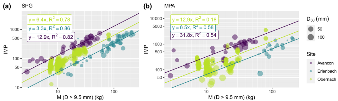
Figure 6. IMP vs. total transported mass M ( D > 9.5 mm) for the calibration measurements at different sites. Samples lighter than 5 kg were excluded for the calculation of the regression for the Avançon de Nant. Results in panel (a) are for the SPG, and results in panel (b) are for the MPA.
