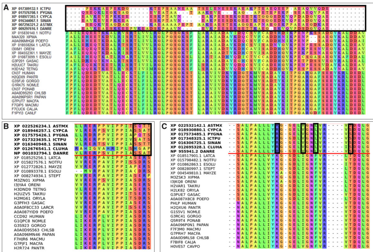
Fig. 7. —Examples of differential conservation detected by BLUR. Comparison was done between two groups of Actinopterygii, Otomorpha (above the red line), and Euteleostomorpha (below the red line). Homo sapiens was used as a query species, the multiple sequence alignments contain sequences of mammals. (A) Multiple sequence alignment of CNP. Differential conservation of a large region can be seen in protein sequences of Otomorpha. (B) Multiple sequence alignment of CCDC92. Differential conservation of a small motif can be seen in protein sequences of Otomorpha. (C) Multiple alignment of PDCL. Differential conservation of single amino acids can be observed in protein sequences of Otomorpha.
