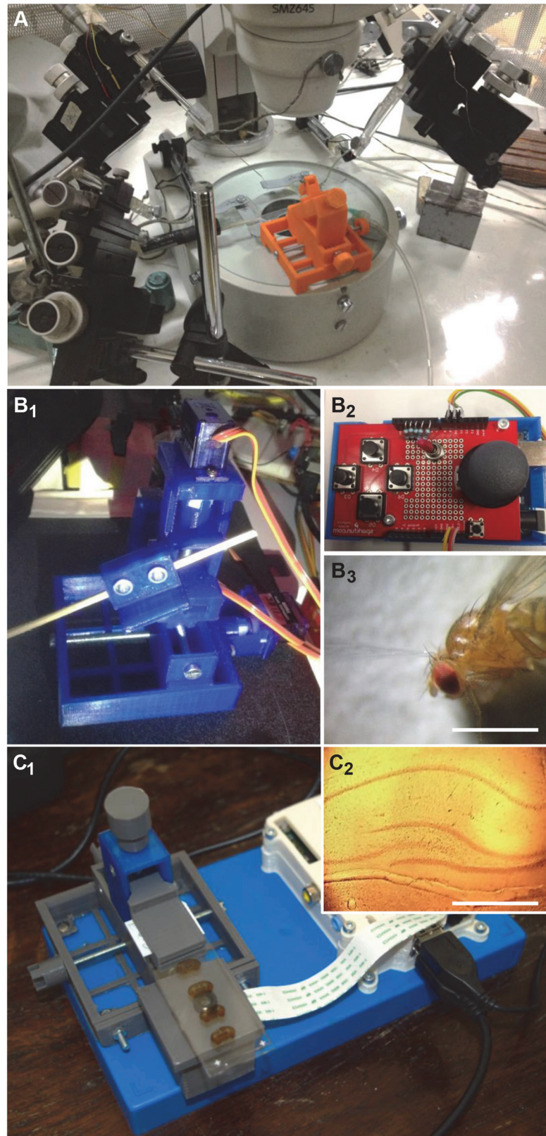
Fig 2. Evolution of an Open Labware design. A , A 3-D printable micromanipulator with a slanted Z-axis [18], here shown amidst commercial alternatives, initially served as the basis for a motorized version with
