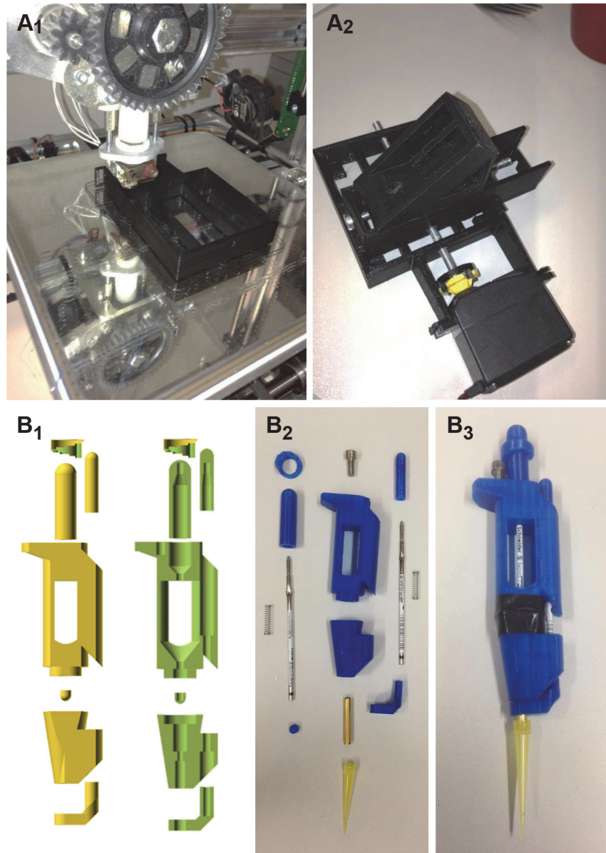
Fig 1. Examples of open 3-D printed laboratory tools. A 1 , Components for laboratory tools, such as the base for a micromanipulator [18] shown here, can be rapidly prototyped using 3-D printing. A 2 , The printed parts can be easily combined with an off-the-shelf continuous rotation servo-motor (bottom) to motorize the main axis. B 1 , A 3-D printable micropipette [8], designed in OpenSCAD [19], shown in full (left) and cross-section (right). B 2 , The pipette consists of the printed parts (blue), two biro fillings with the spring, an off-the-shelf piece of tubing to fit the tip, and one screw used as a spacer. B 3 , Assembly is complete with a laboratory glove or balloon spanned between the two main printed parts and sealed with tape to create an airtight bottom chamber continuous with the pipette tip. Accuracy is \pm 2\text{--}10\ \mu\text{l} depending on printer precision, and total capacity of the system is easily adjusted using two variables listed in the source code, or accessed via the “Customizer” plugin on the thingiverse link [8]. See also the first table.
