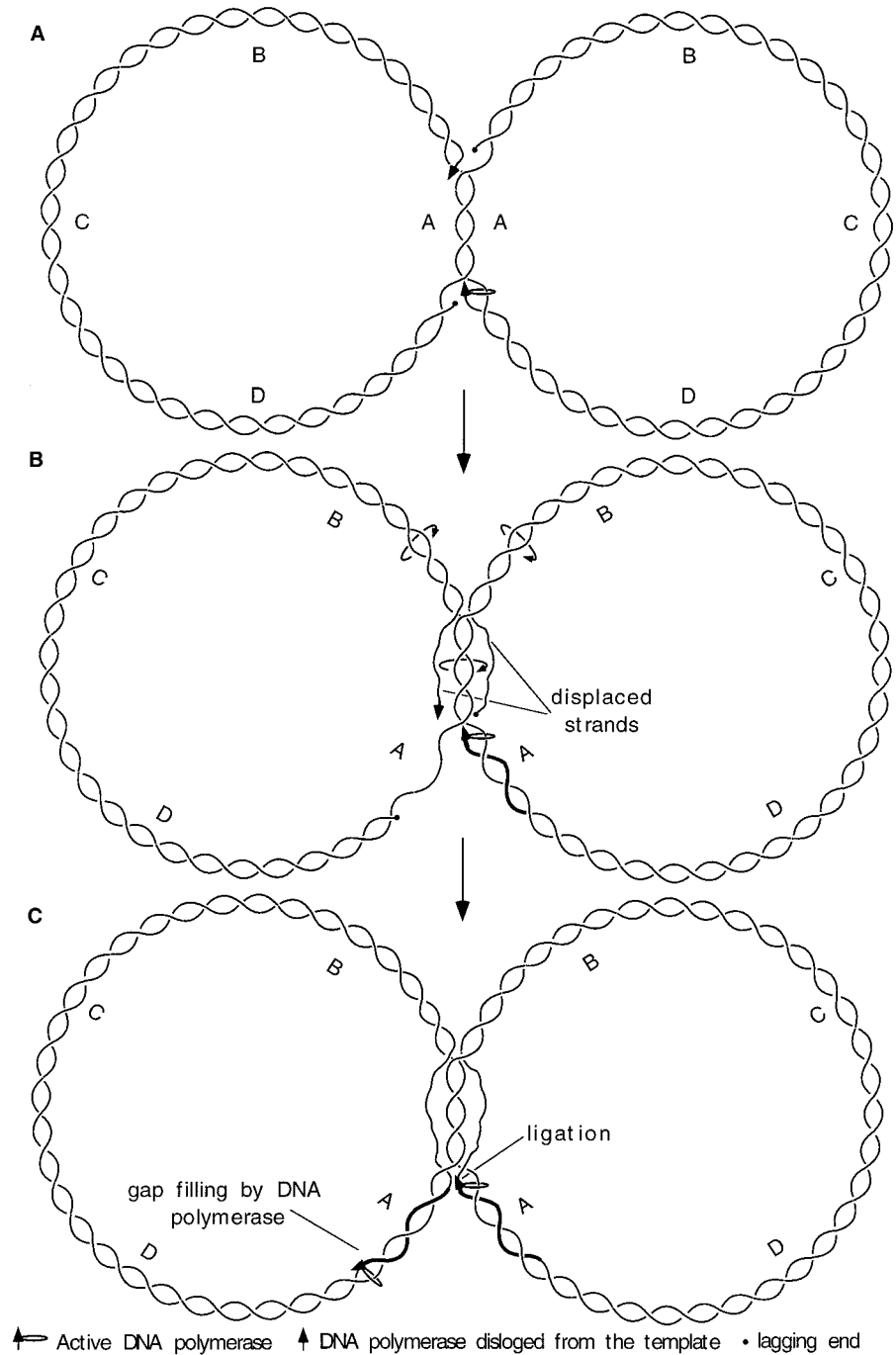
FIGURE 6 Termination of circular DNA replication via hemicatenation. (A) Cairns' structure with two remaining interlockings. In one of the forks, DNA polymerase becomes dislodged from the template. (B) Active DNA polymerase in the lower fork induces axial rotation and branch migration of the region of interlockings. This causes progressive displacement of leading and lagging strands from the other replication fork. A newly synthesized DNA strand is drawn with a thick line. Notice that the two interlocked molecules changed locations of the interlockings. (C) Upon reannealing of both displaced ends with the corresponding single-stranded regions exposed in the replication fork, the synthesis of both complementary strands can be terminated. The resulting hemicatenane is interlocked by the parental strands.
