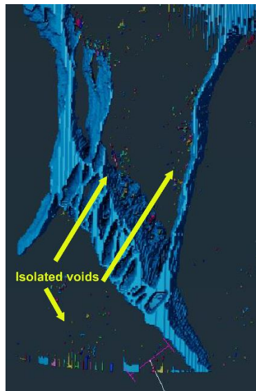
Figure 58 Visualization of 3D fracture network reconstructed were the voids that are not connected with the external boundaries are indicated (AVIZO™)
