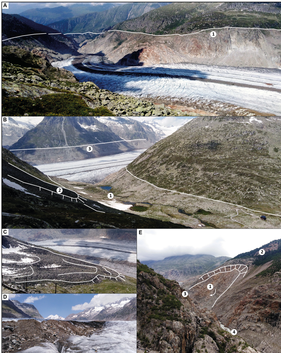
Fig. 4. A. Snout of the Great Aletsch Glacier. The white line indicates its maximum LIA position, highlighted by contrasts of colours and vegetation (1). B. The former Märjelen Lake (1) with its maximum extension. A rock glacier (2) and the LIA limits of the Great Aletsch Glacier (3) are also visible. C. Grosses Gufer Rock Glacier. D. A medial moraine of the Great Aletsch Glacier. E. Moosfluh instability, with zones affected by rotational sliding (1) and by toppling movement (2) after the retreat of the glacier (3). Basal erosion by the Massa River (4) could cause a renewed acceleration of the entire landslide. Photos: Jonathan Bussard, 2021.
