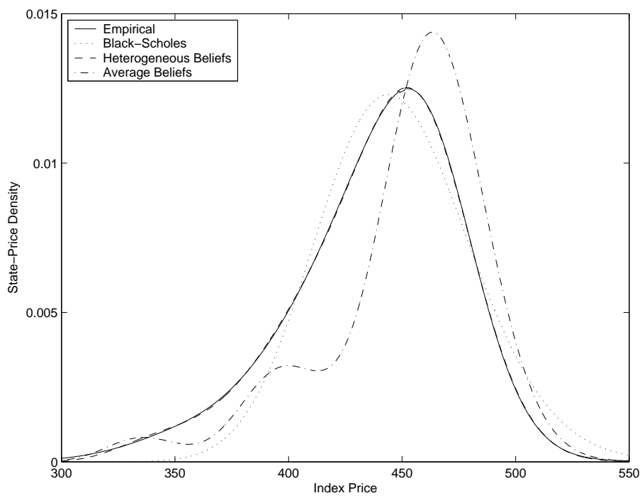
Figure 7: CRRA state-price density with heterogeneous beliefs
