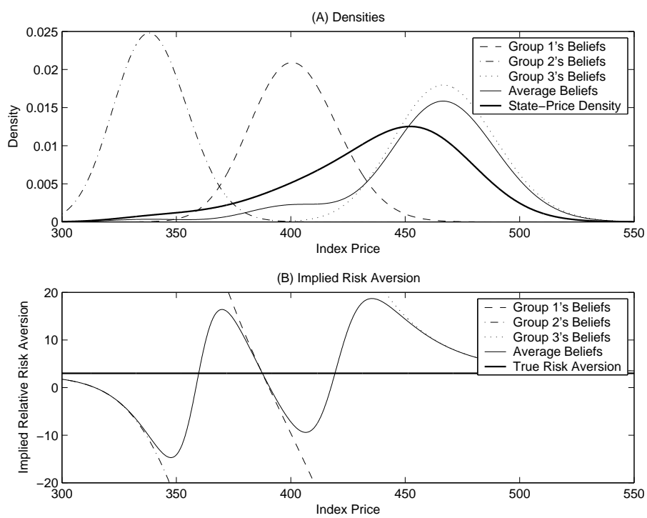
Figure 8: CRRA state-price density with heterogeneous beliefs: density and implied risk aversion estimates
