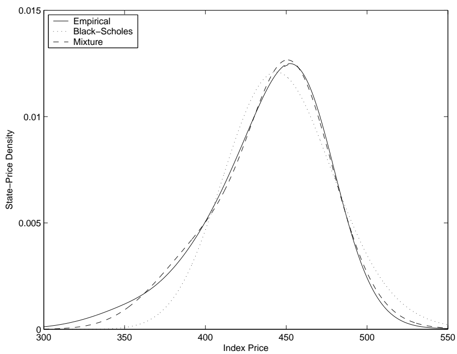
Figure 3: A Peso problem: CRRA state-price density with a mixture of lognormal distributions
