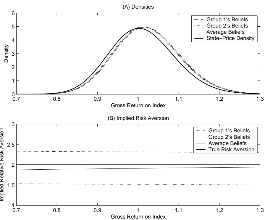
Figure 4: Heterogeneous beliefs and implied risk aversion – small heterogeneity
