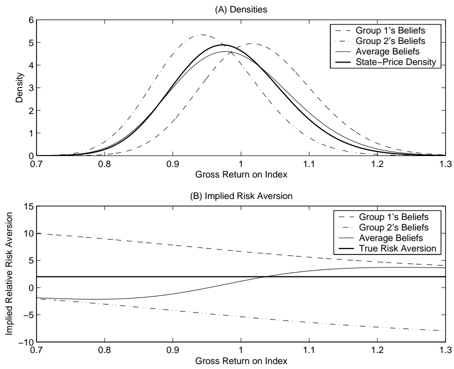
Figure 5: Heterogeneous beliefs and implied risk aversion – large heterogeneity
