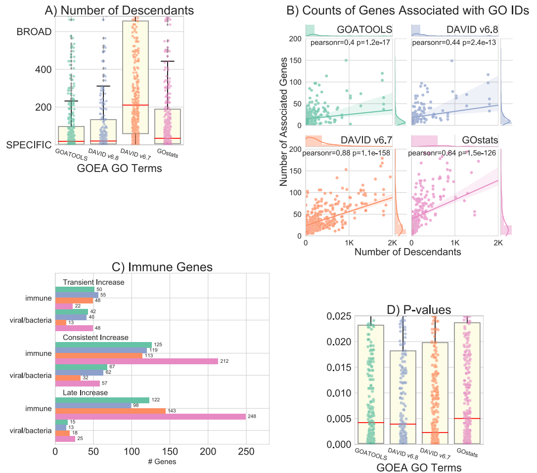
Figure 5. Comparison between enriched terms identified by GOATOOLS, DAVID and Gostats. All panels use the the same color coding as specified in the legend in Fig. 4. (A) Number of descendants for the significant terms reported in GOATOOLS, DAVID6.7, DAVID6.8, and Gostats. GOATOOLS and DAVID6.8 both discovered GO IDs with the lowest and most similar specificity. Gostats median GO ID broadness was twice that of GOATOOLS and DAVID6.8. DAVID6.7 discovered GO IDs 10x as broad as GOATOOLS when using mean dcnt . (B) Broader GO terms are associated with more genes while specific GO terms are associated with fewer genes. All four tools show a positive correlation between descendants count and the number of genes associated with the GO term. GOATOOLS and the most recent DAVID generally discovered very specific GO IDs associated with fewer genes. DAVID6.7 and Gostats found broader GO IDs that were associated with large numbers of genes. (C) Clusters and counts of genes significant for terms related to immunity. GOATOOLS and DAVID6.8 are most similar in the types and numbers of genes discovered. GOATOOLS discovered genes significant in immune and viral/bacterial categories for all GP clusters contrasted to the DAVID6.7 which found no viral/bacteria genes for any cluster. Gostats often found more genes, but they were often associated with broad GO IDs. (D) Comparison of P-values for all of the GO terms found in total in all four tools. The mean P-values were similar for GOATOOLS, DAVID6.8, and Gostats. DAVID6.7 had P-values multitudes lower than all the other tools.
